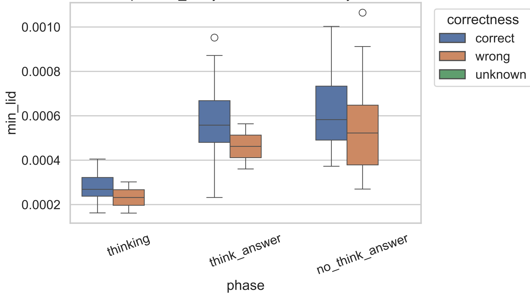
Exp C min_lid by correctness, 32B, layer 6
