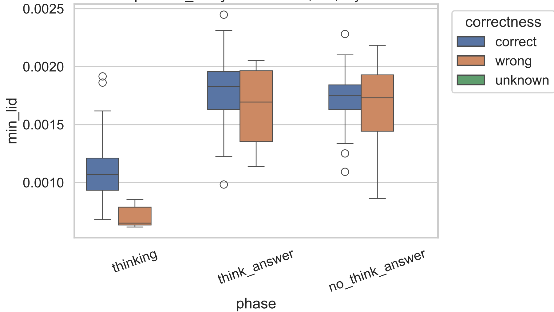
Exp C min_lid by correctness, 4B, layer 13
