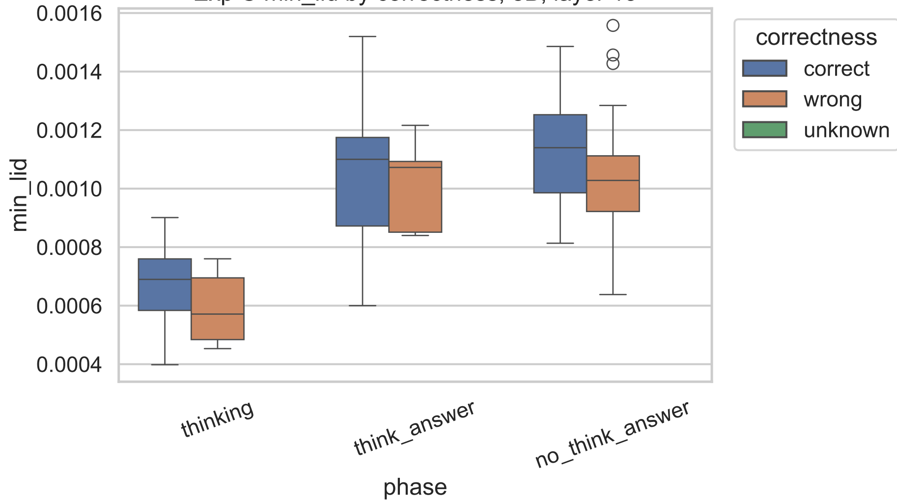
Exp C min_lid by correctness, 8B, layer 13
