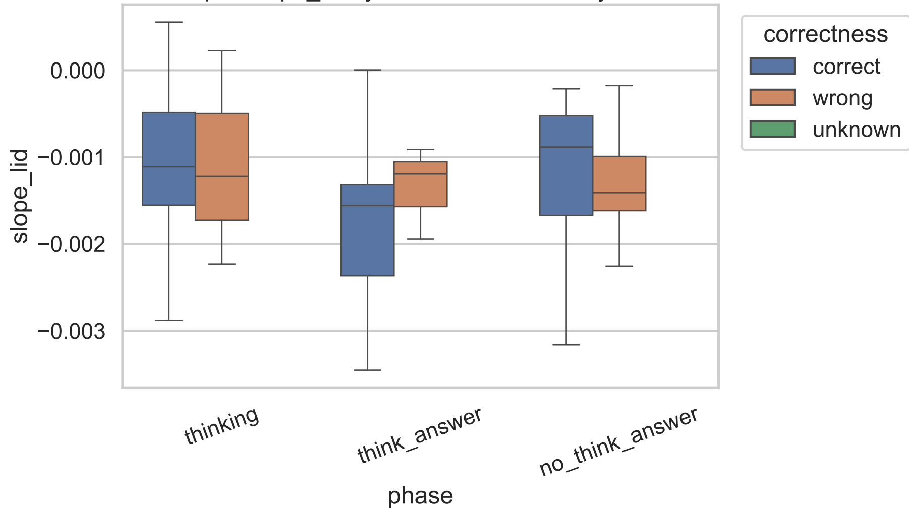
Exp C slope_lid by correctness, 14B, layer 13
