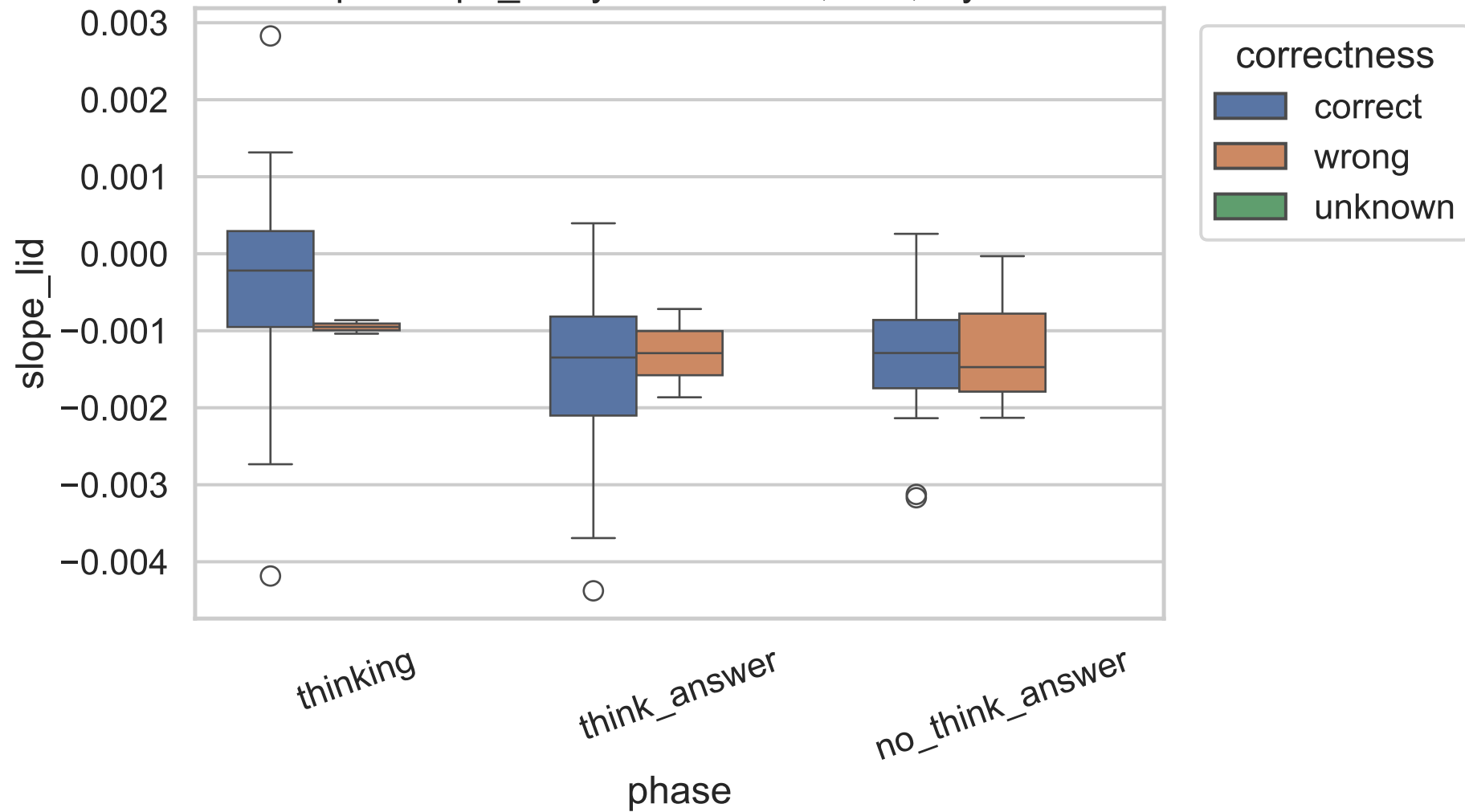
Exp C slope_lid by correctness, 32B, layer 13
