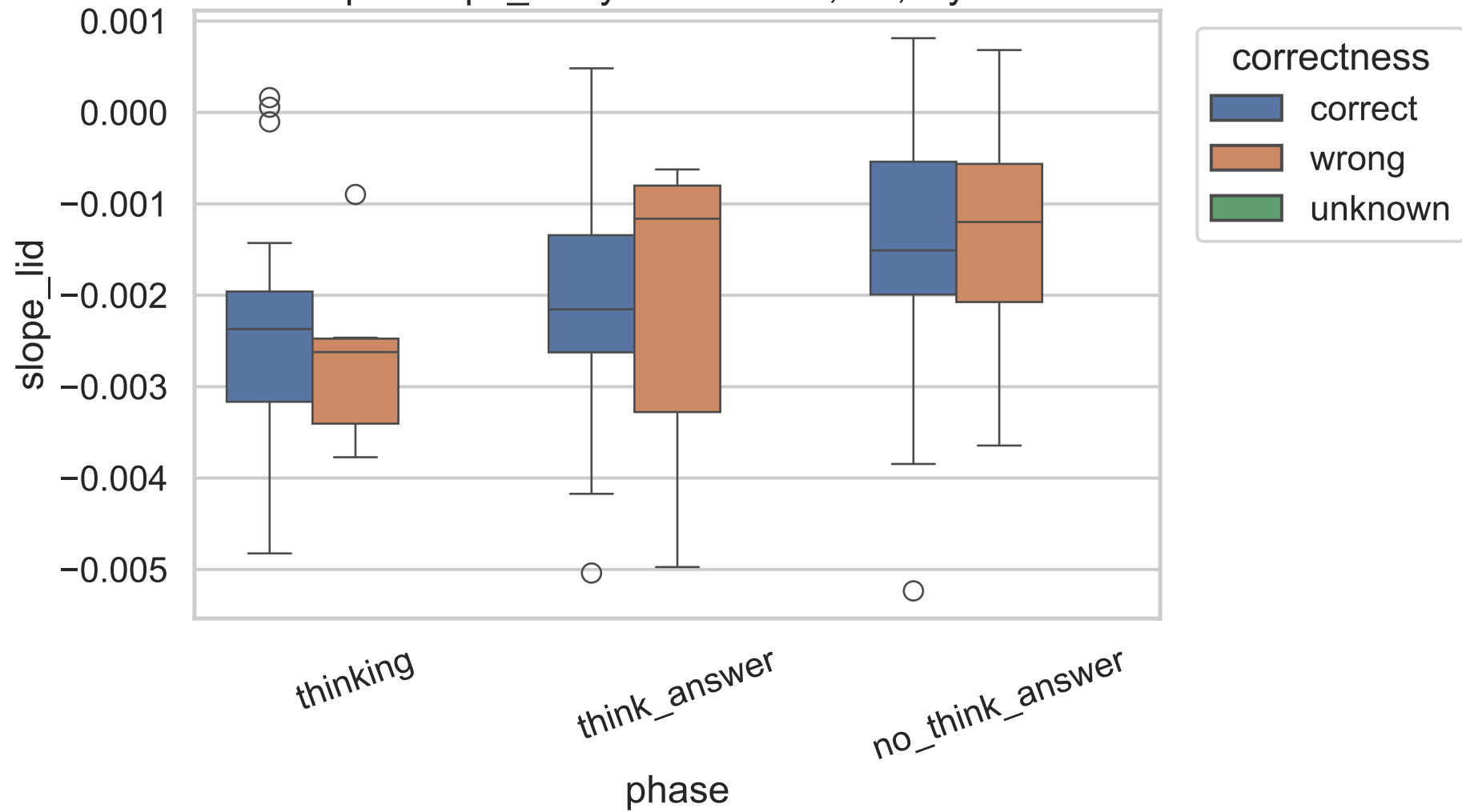
Exp C slope_lid by correctness, 4B, layer 13
