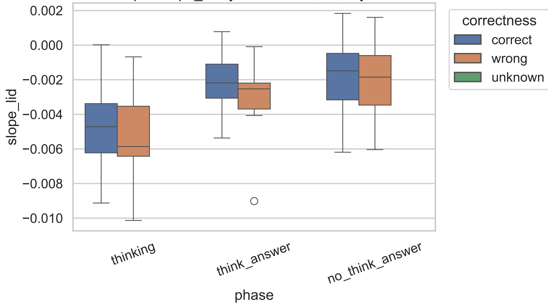
Exp C slope_lid by correctness, 4B, layer 6
