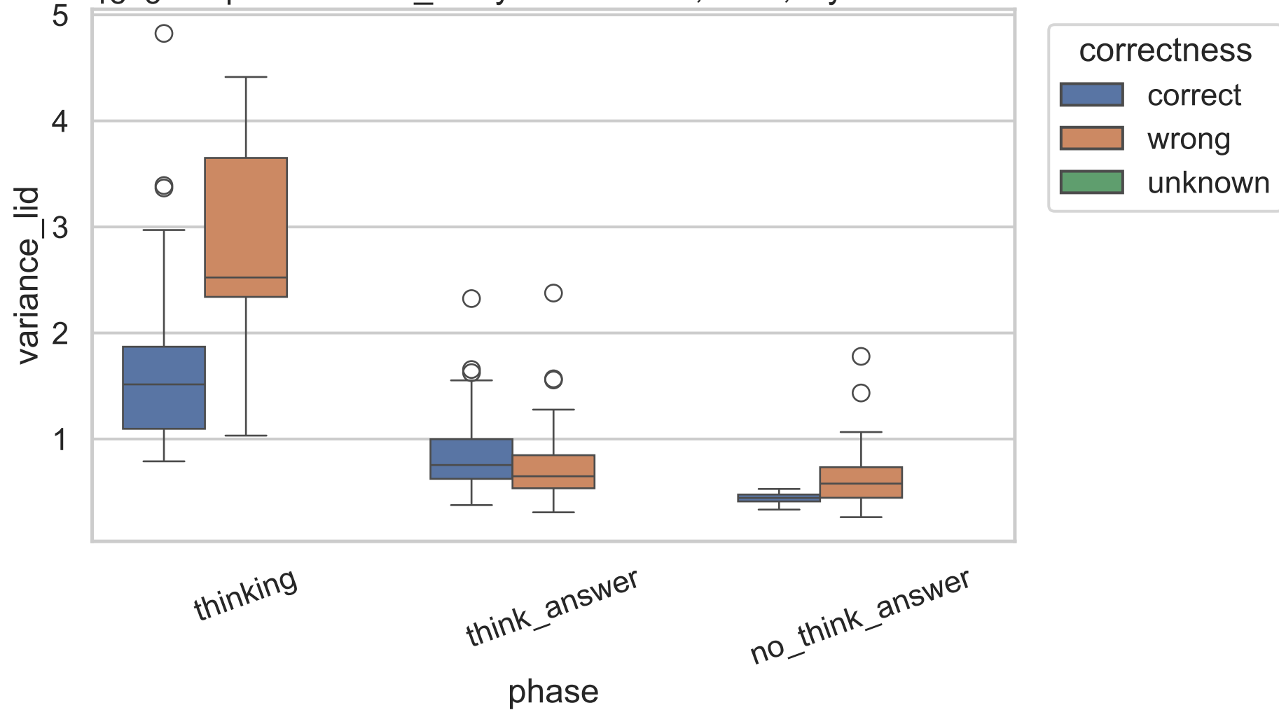
1e-5 Exp C variance_lid by correctness, 1.7B, layer 13
