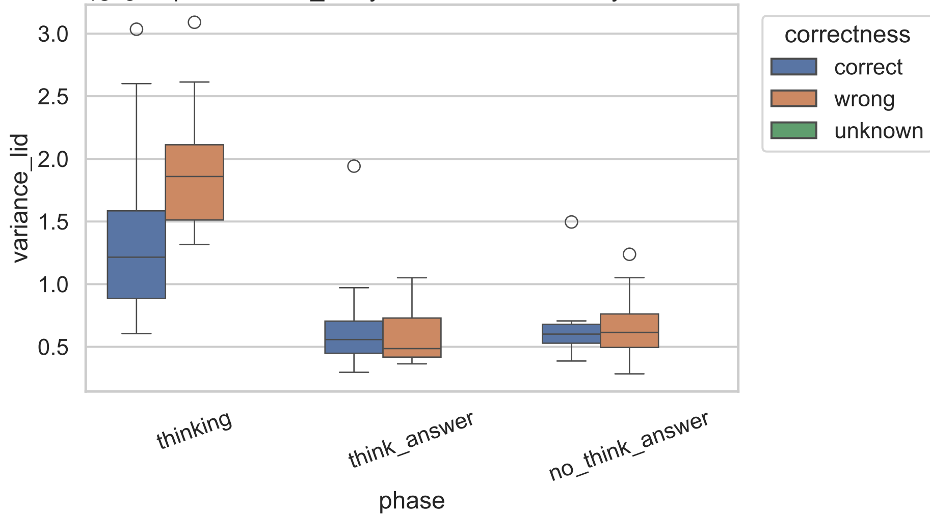
1e-5 Exp C variance_lid by correctness, 1.7B, layer 20
