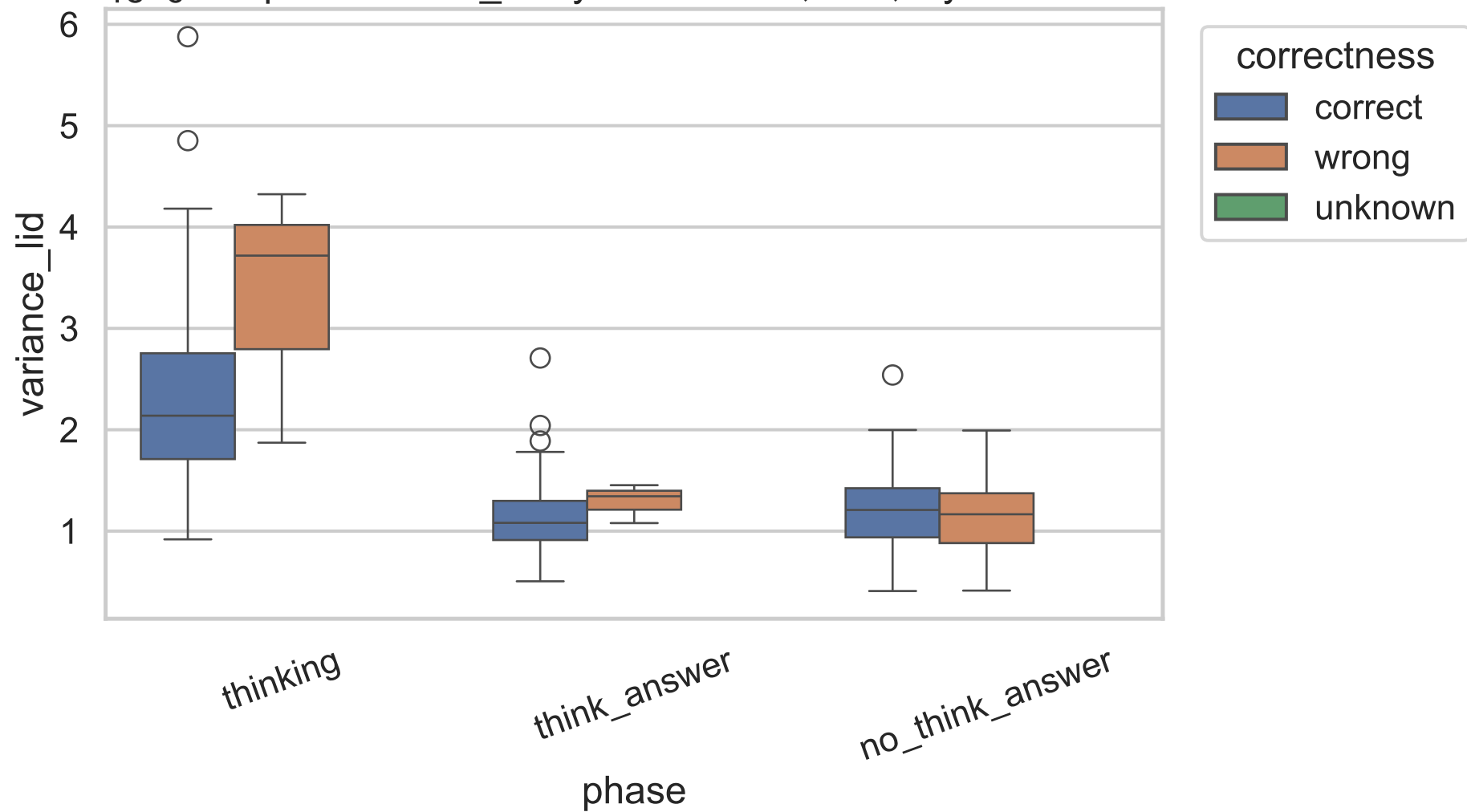
1e-6 Exp C variance_lid by correctness, 14B, layer 20
