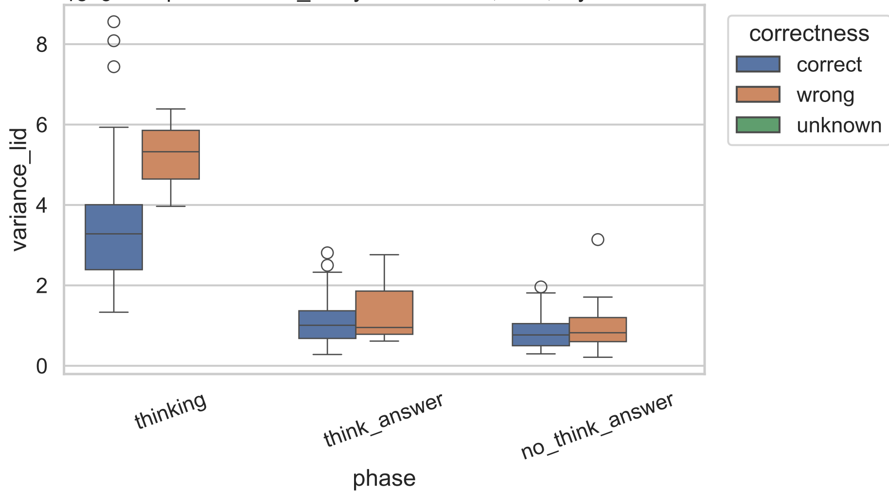
1e-5 Exp C variance_lid by correctness, 14B, layer 6
