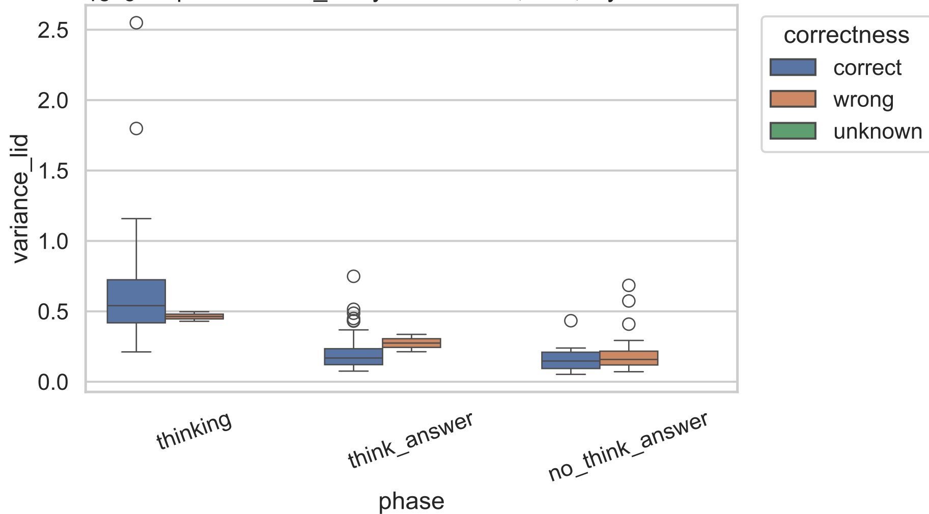
1e-5 Exp C variance_lid by correctness, 32B, layer 20
