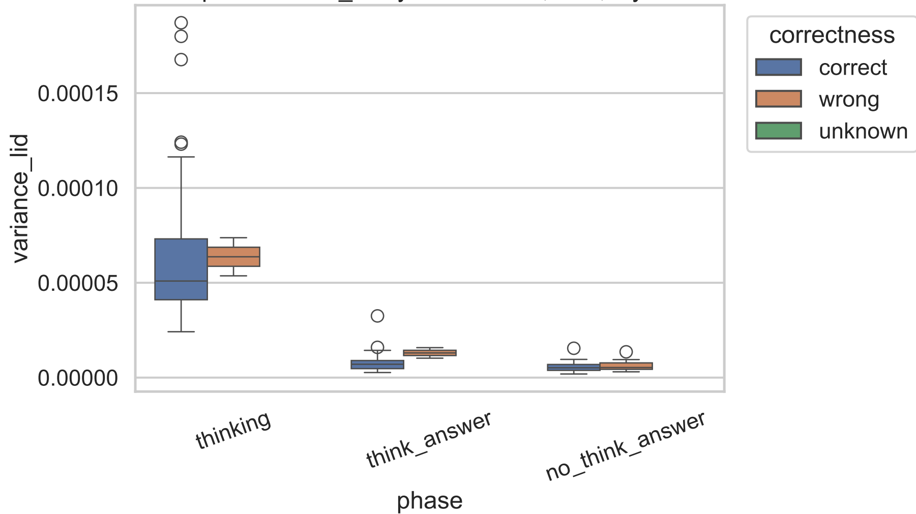
Exp C variance_lid by correctness, 32B, layer 6
