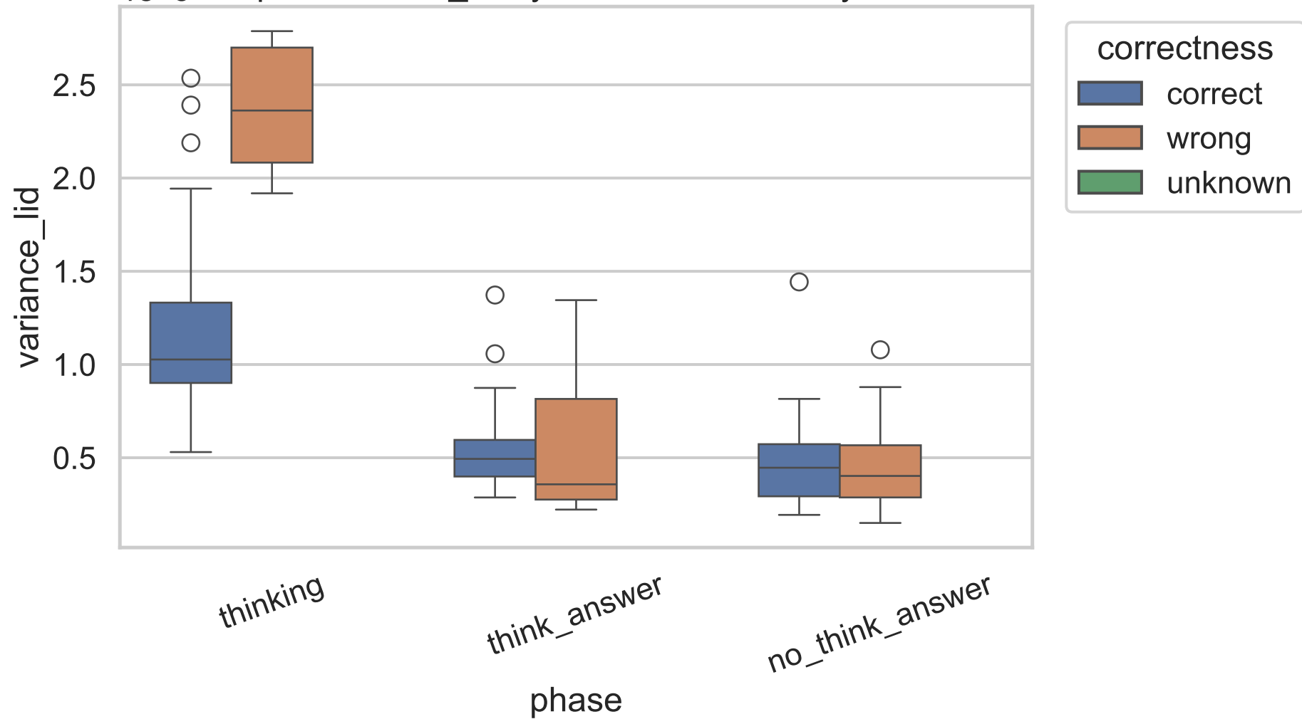
1e-5 Exp C variance_lid by correctness, 4B, layer 13
