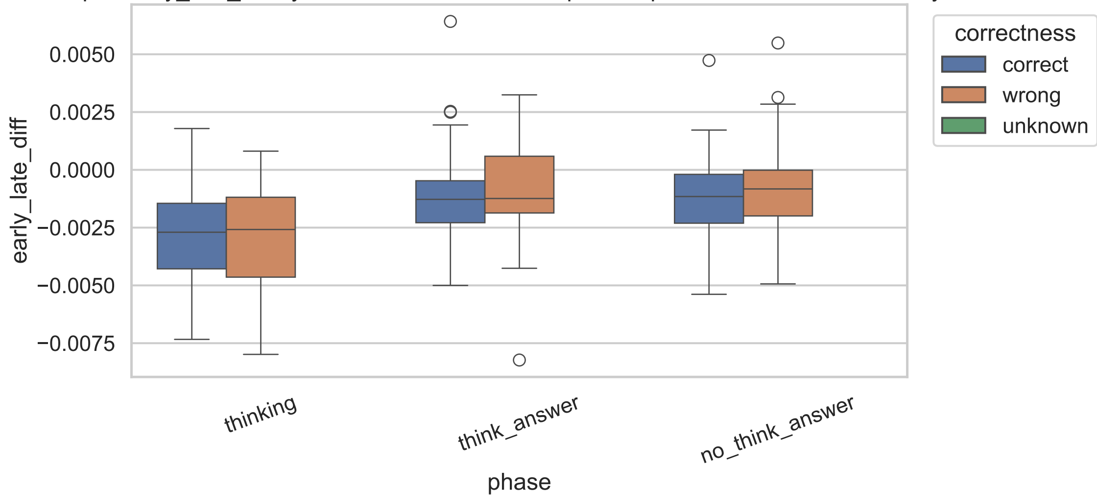
Exp C early_late_diff by correctness, common-kept examples across model sizes, layer 6
