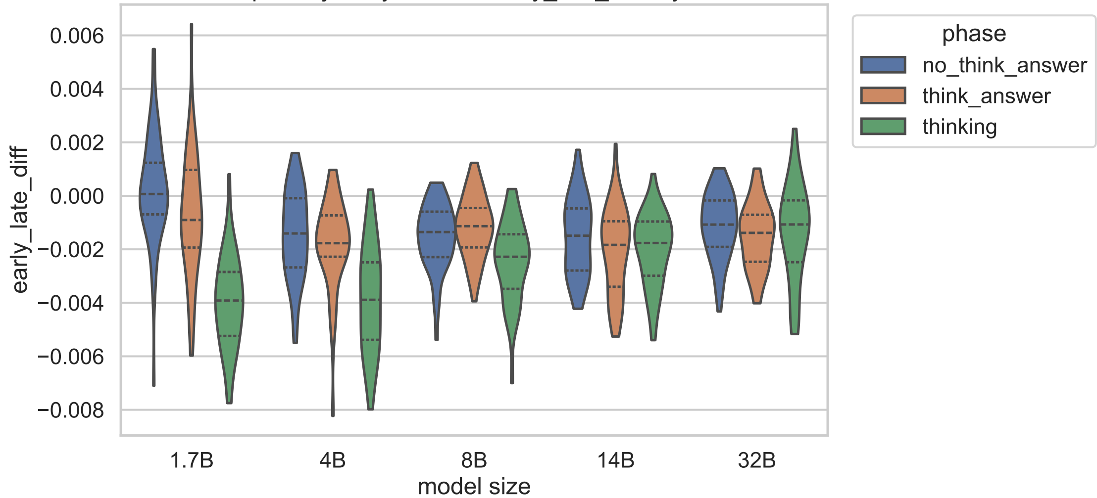
Exp C trajectory statistic: early_late_diff, layer 6
