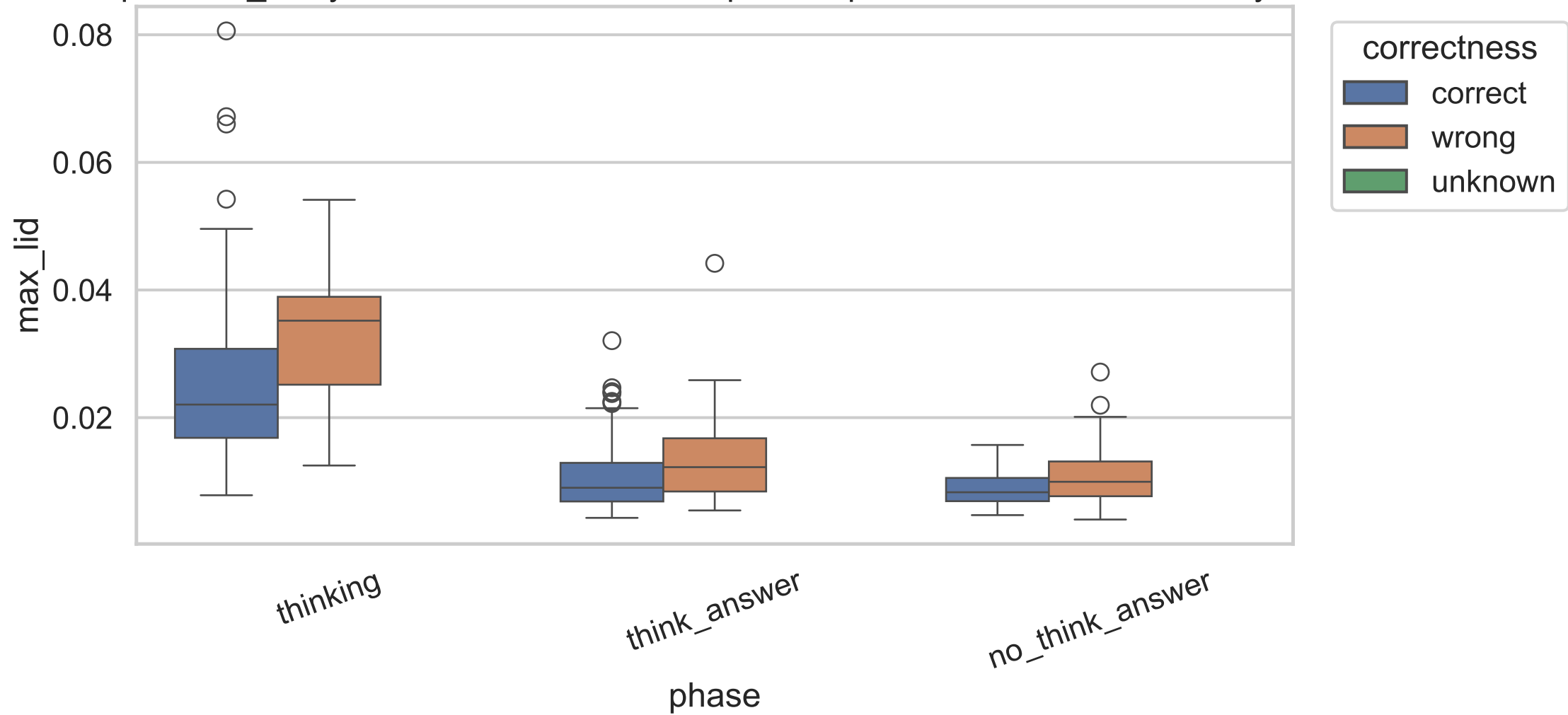
Exp C max_lid by correctness, common-kept examples across model sizes, layer 13
