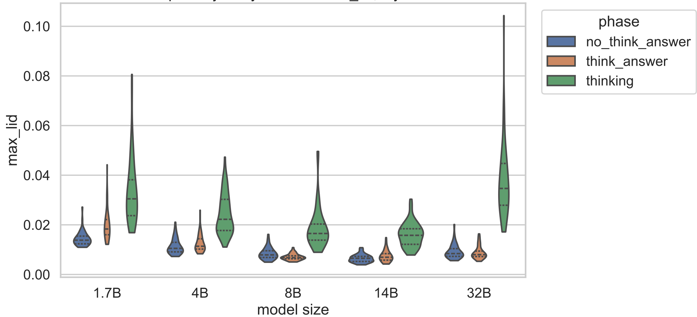
Exp C trajectory statistic: max_lid, layer 13
