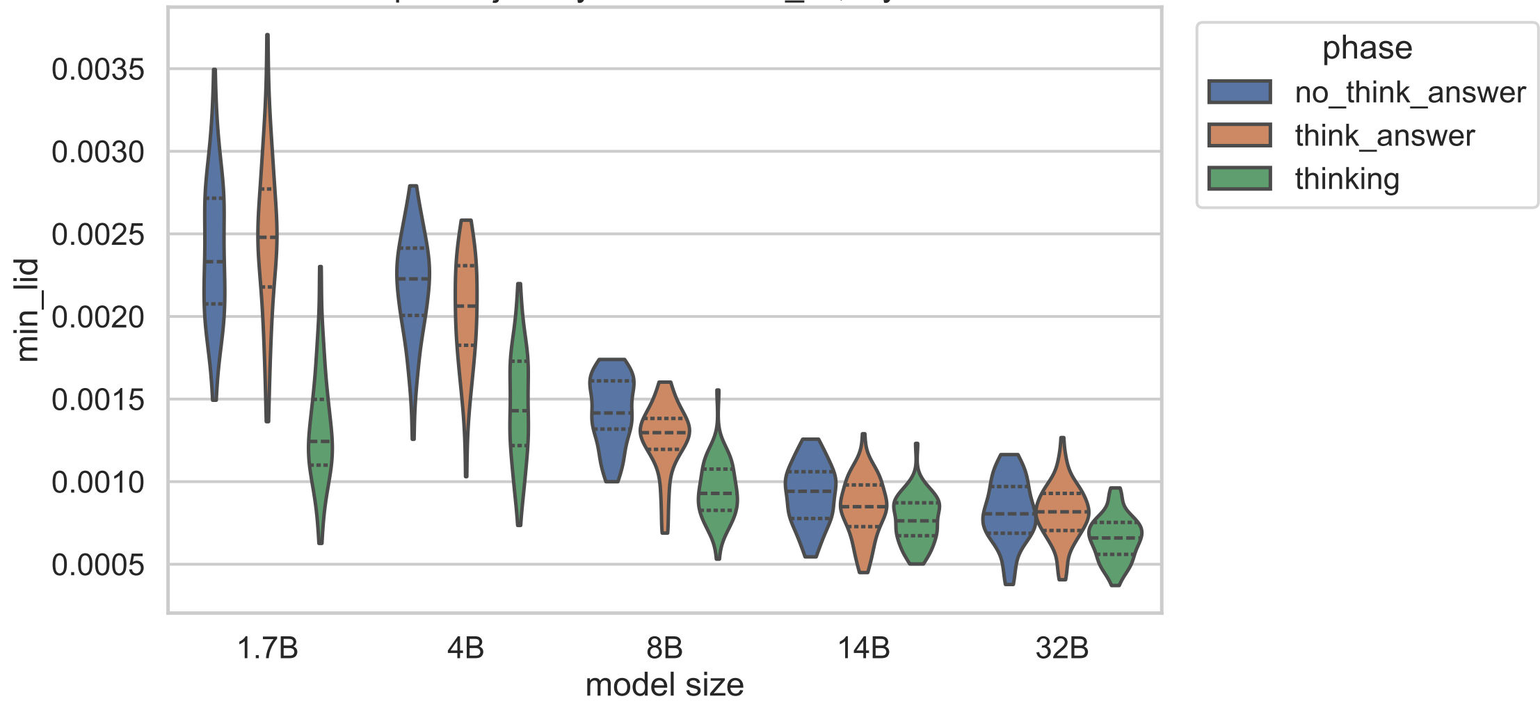
Exp C trajectory statistic: min_lid, layer 20
