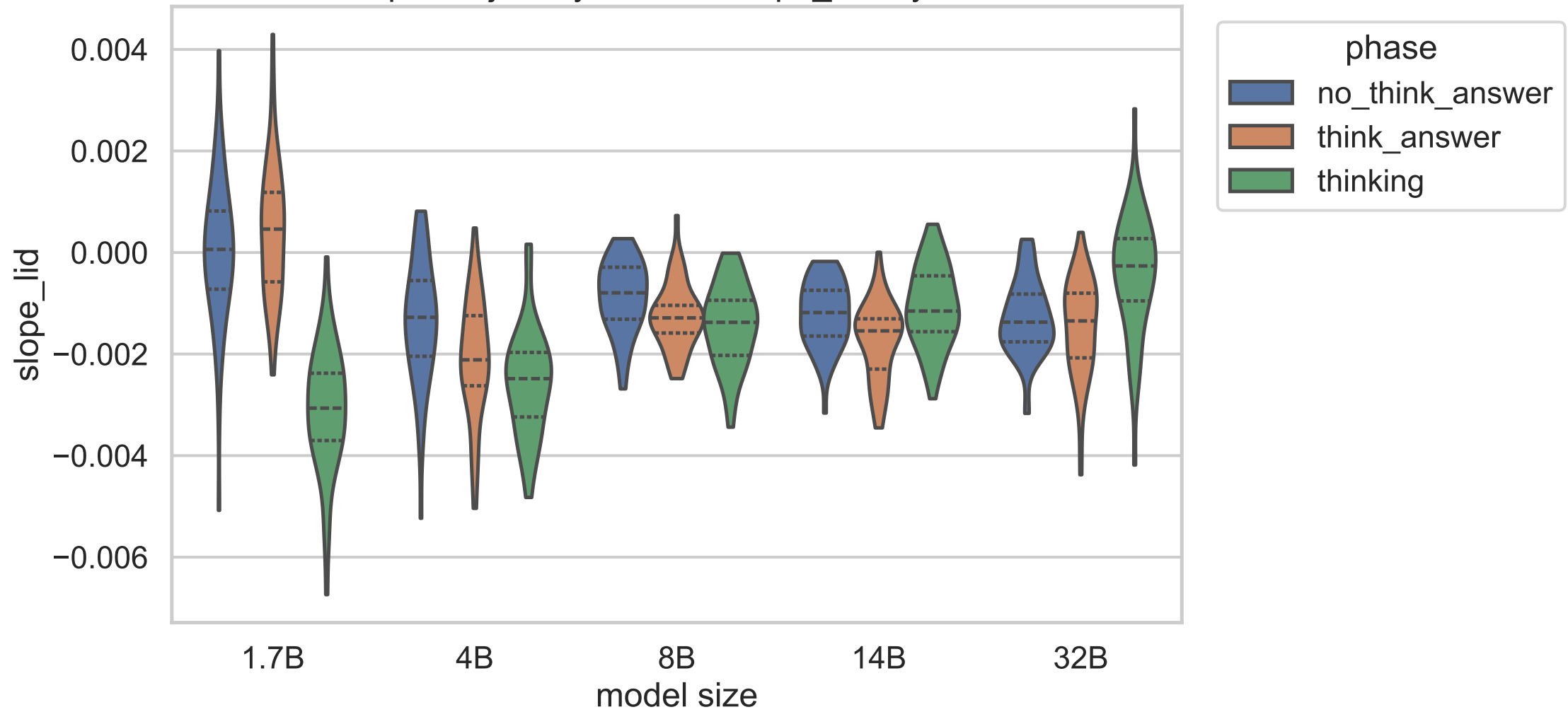
Exp C trajectory statistic: slope_lid, layer 13
