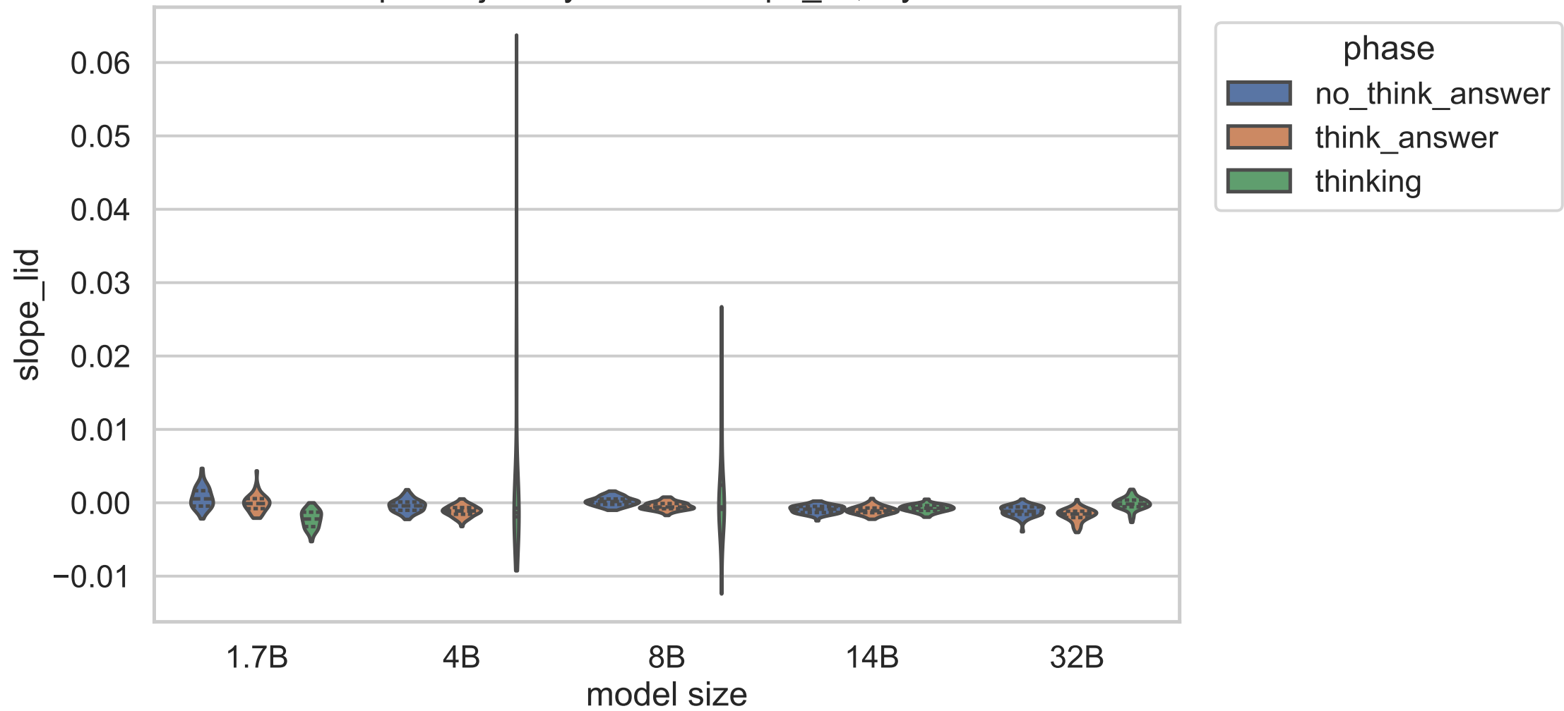
Exp C trajectory statistic: slope_lid, layer 20
