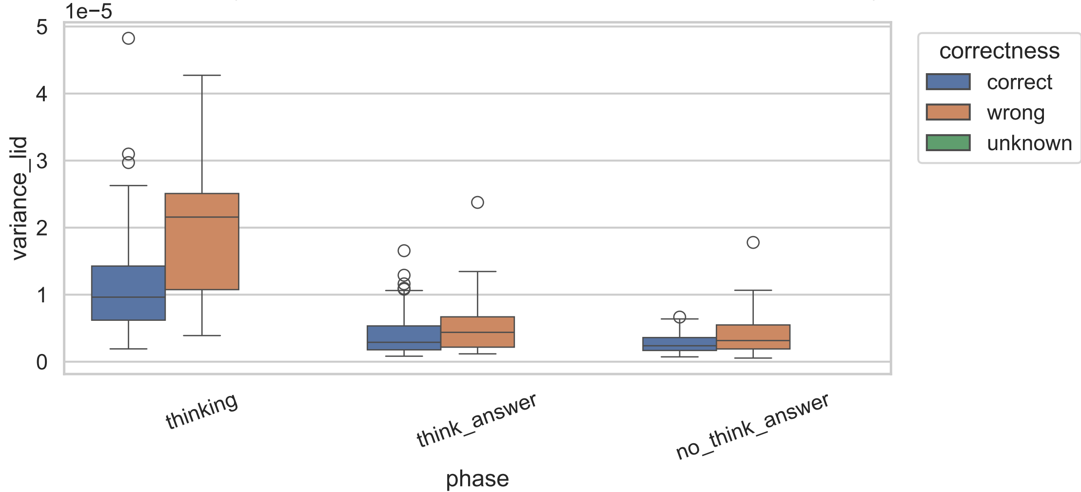
Exp C variance_lid by correctness, common-kept examples across model sizes, layer 13
