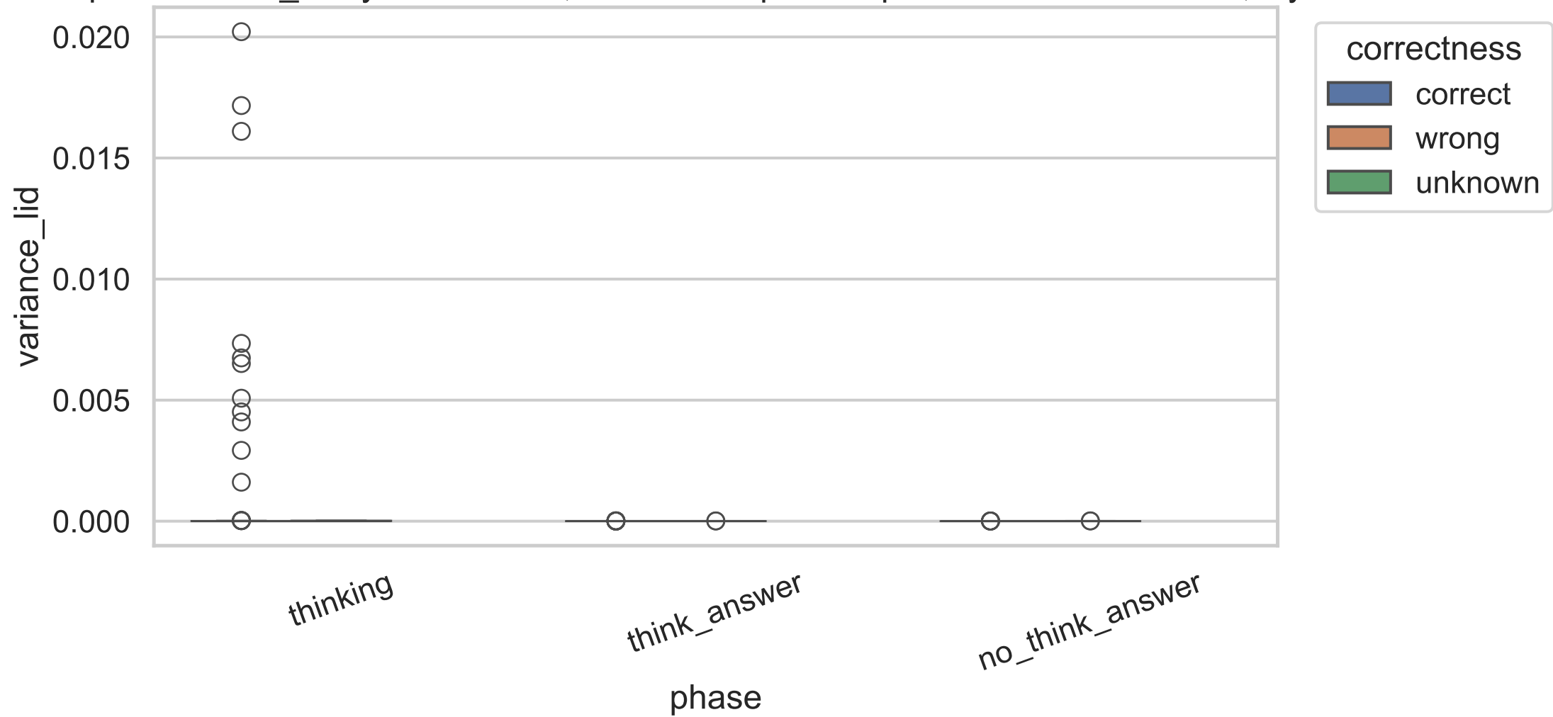
Exp C variance_lid by correctness, common-kept examples across model sizes, layer 20
