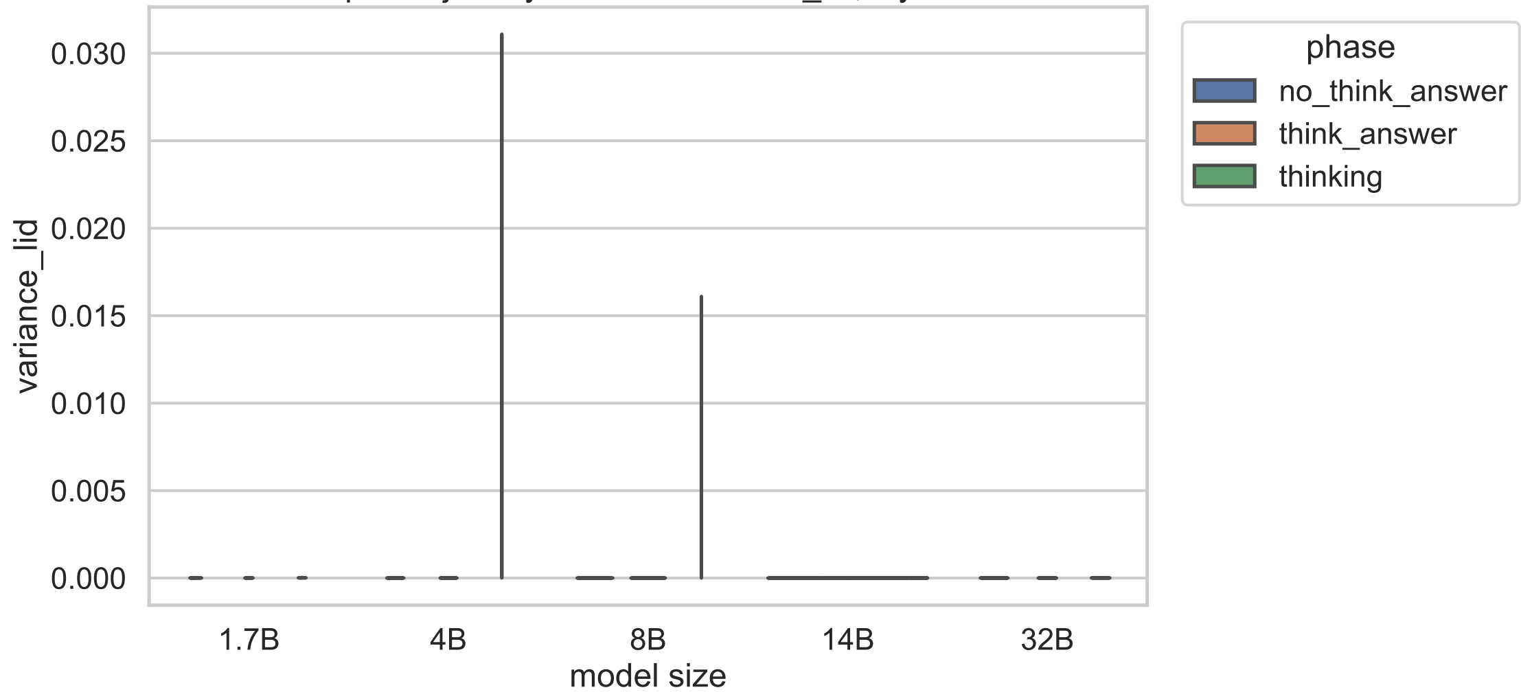
Exp C trajectory statistic: variance_lid, layer 20
