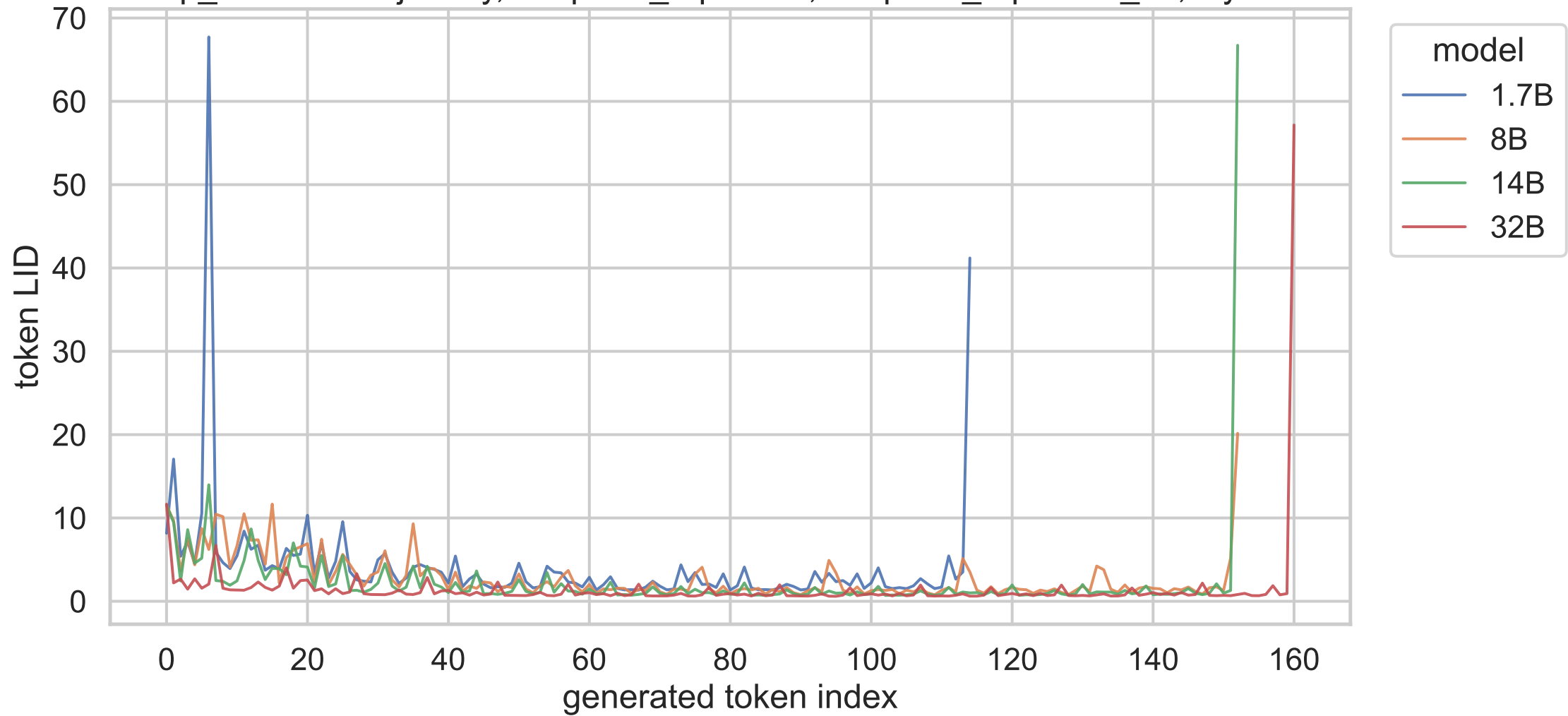
exp_a shared trajectory, templatic_repetition, templatic_repetition_01, layer 13
