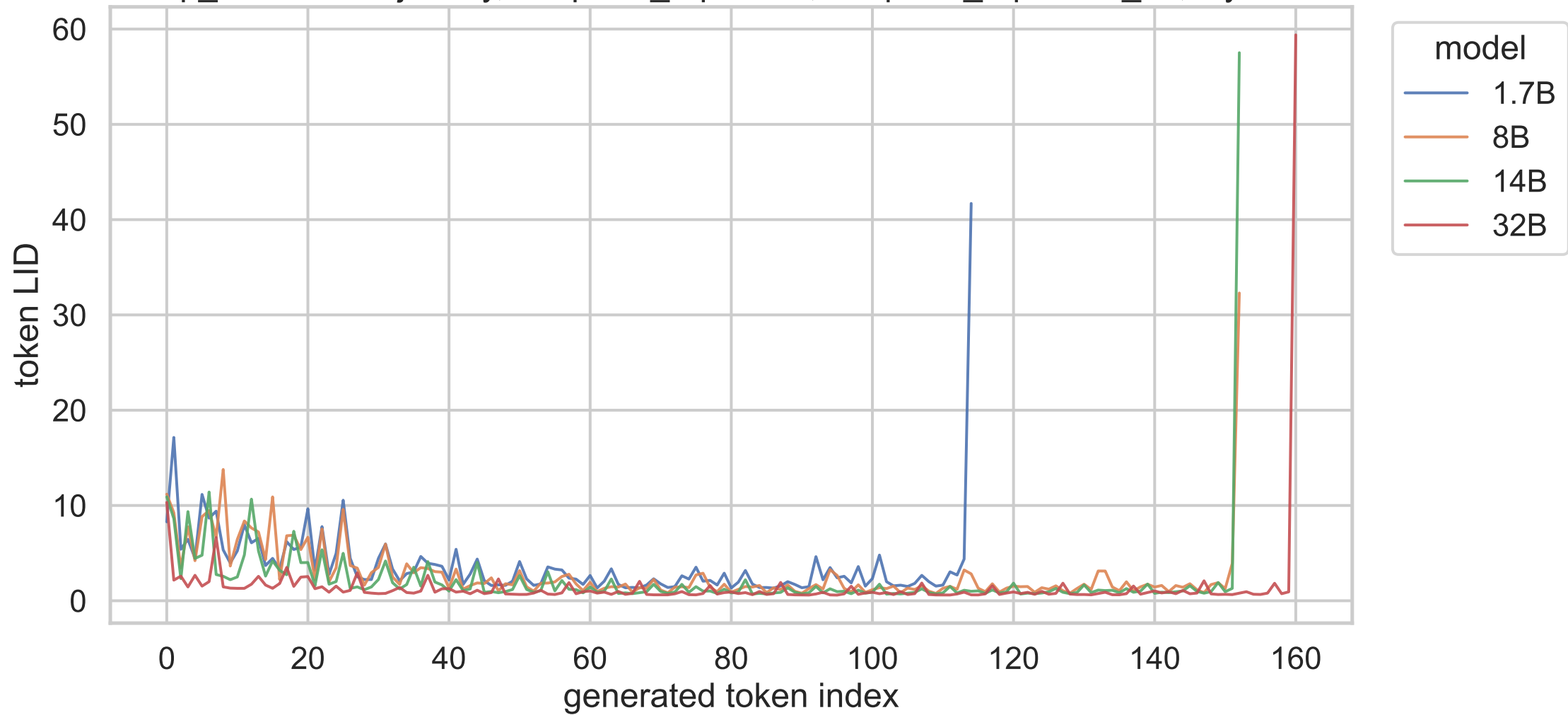
exp_a shared trajectory, templatic_repetition, templatic_repetition_02, layer 13
