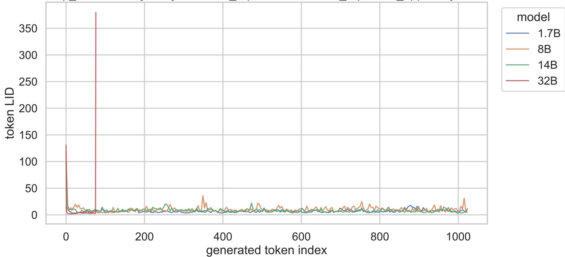
exp_a shared trajectory, constant_repetition, constant_repetition_apple, layer 20
