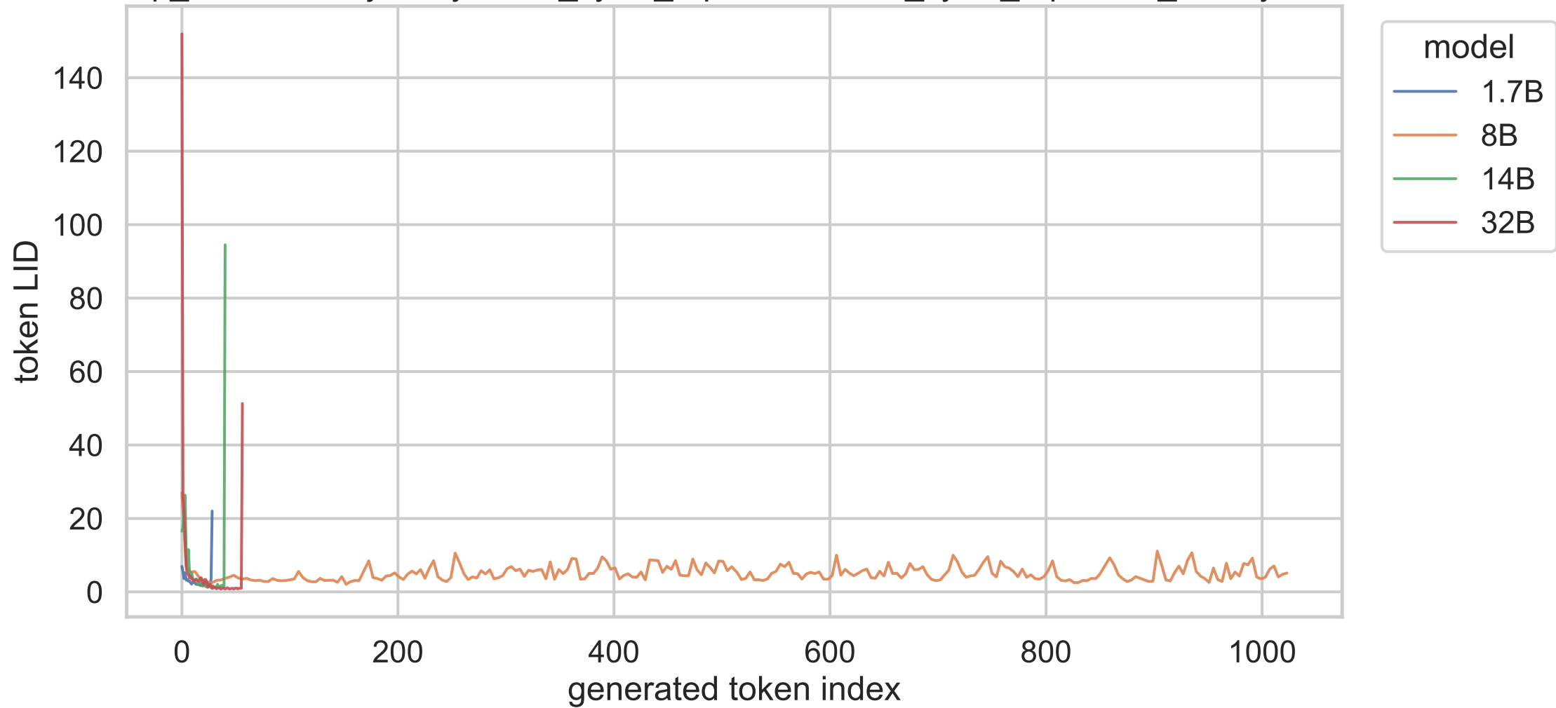
exp_a shared trajectory, short_cycle_repetition, short_cycle_repetition_01, layer 20
