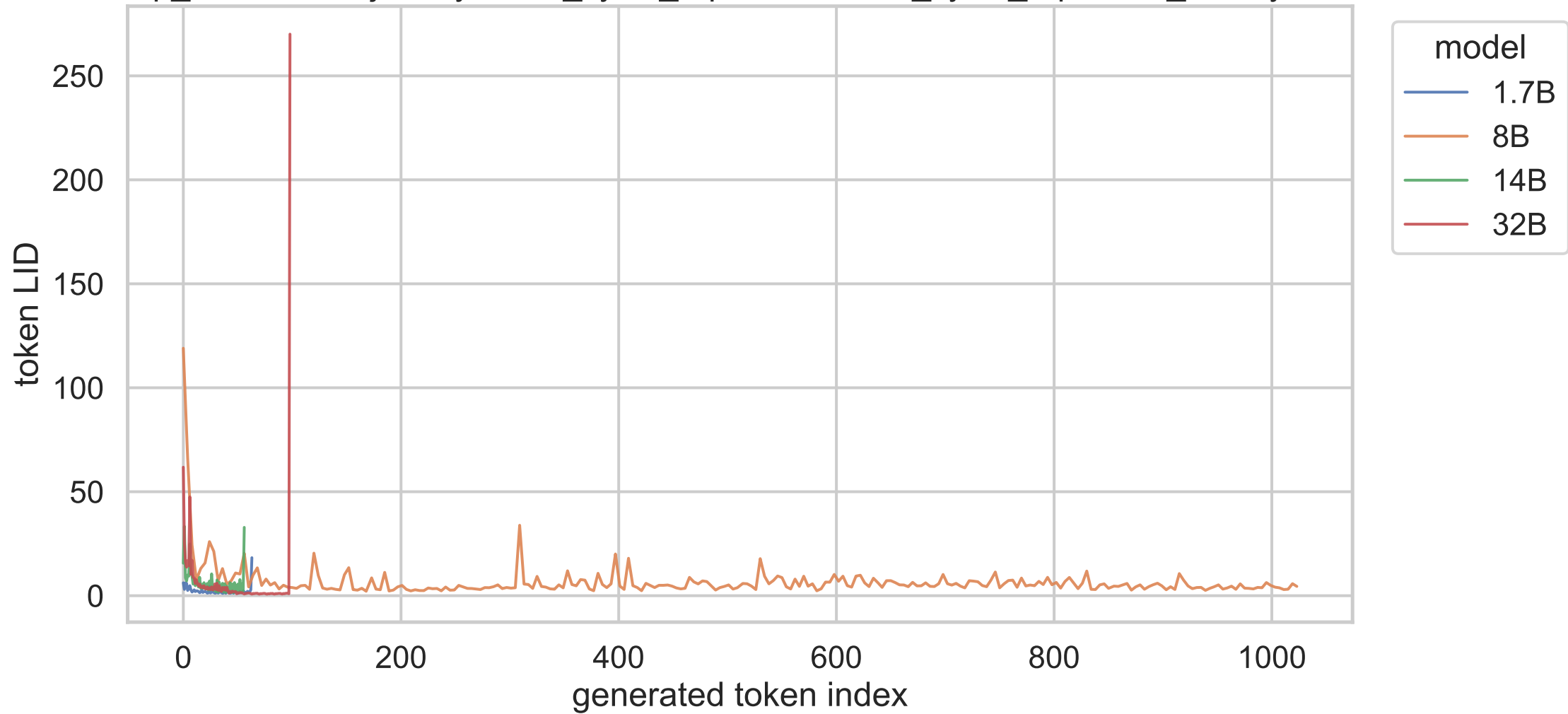
exp_a shared trajectory, short_cycle_repetition, short_cycle_repetition_03, layer 20
