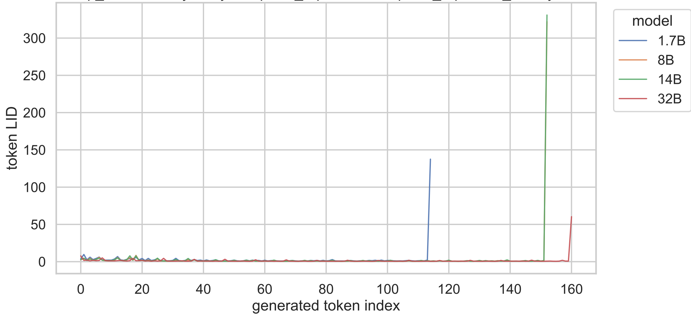
exp_a shared trajectory, templatic_repetition, templatic_repetition_01, layer 6
