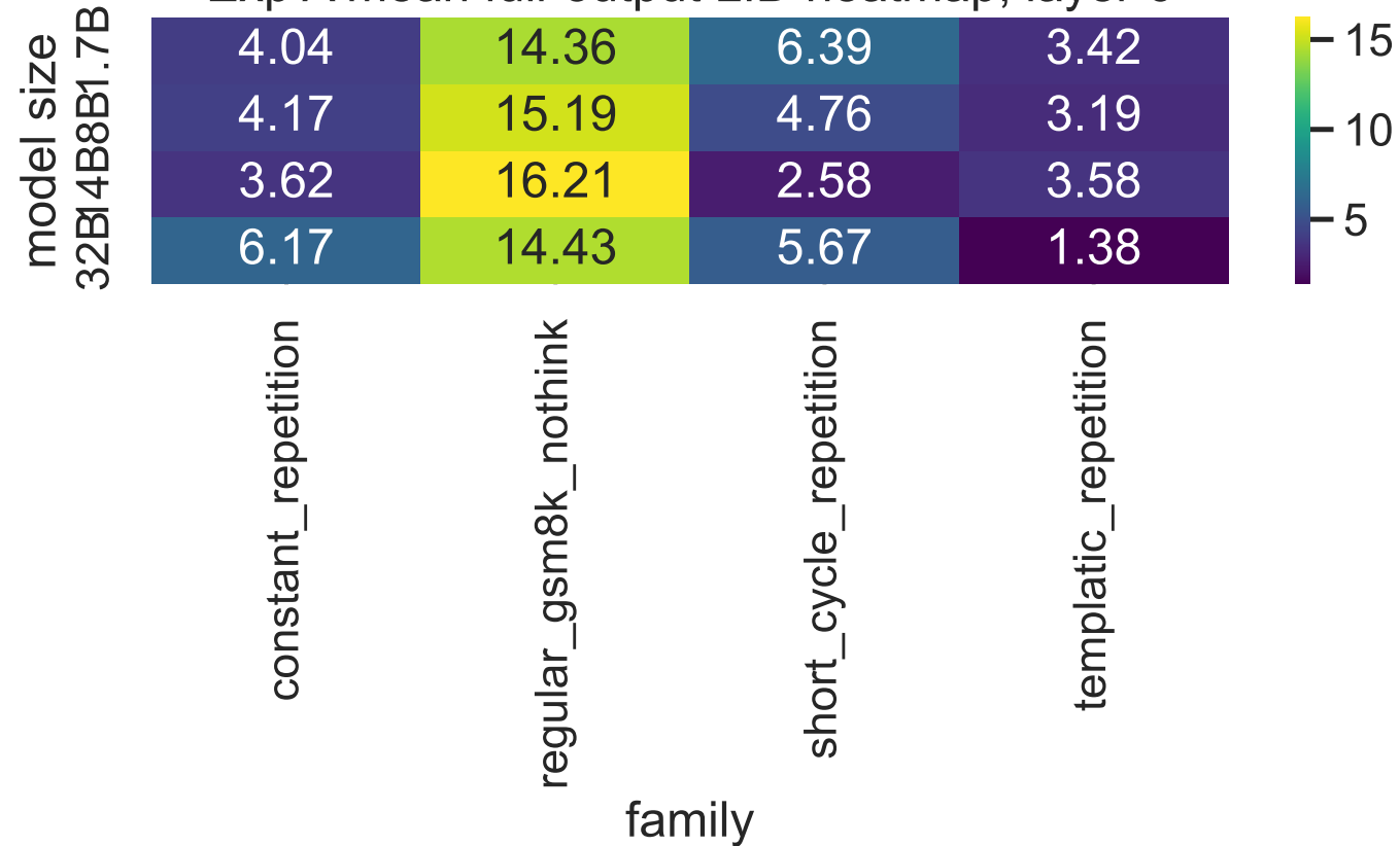
Exp A mean full-output LID heatmap, layer 6
