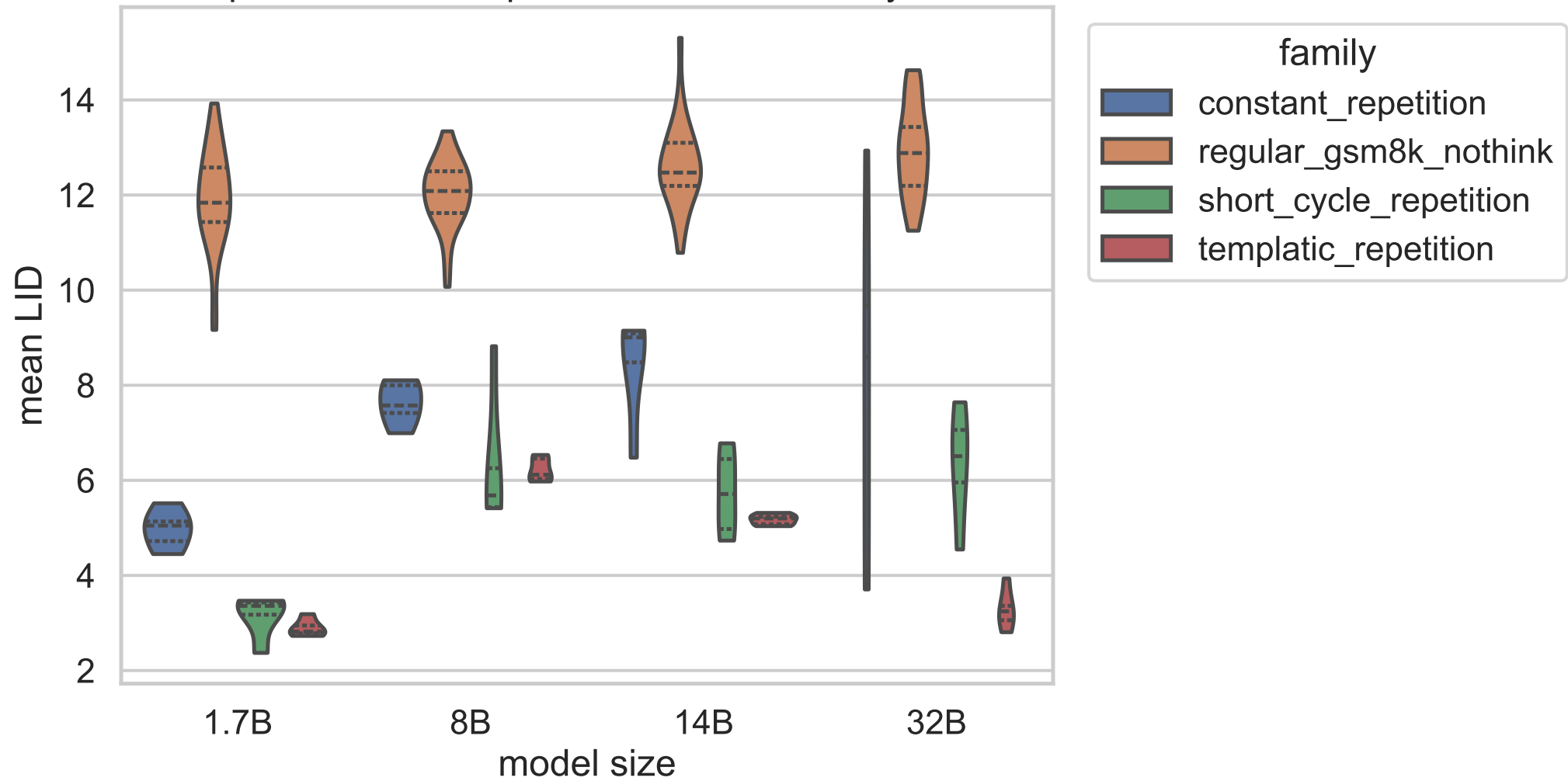
Exp A mean full-output LID distributions, layer 20
