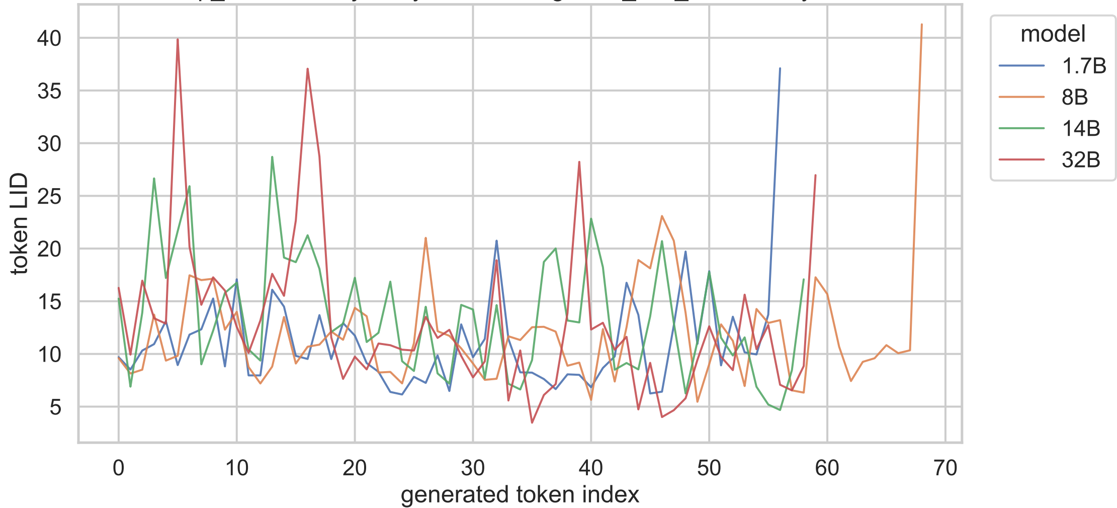
exp_b shared trajectory, canonical, gsm8k_test_000052, layer 20
