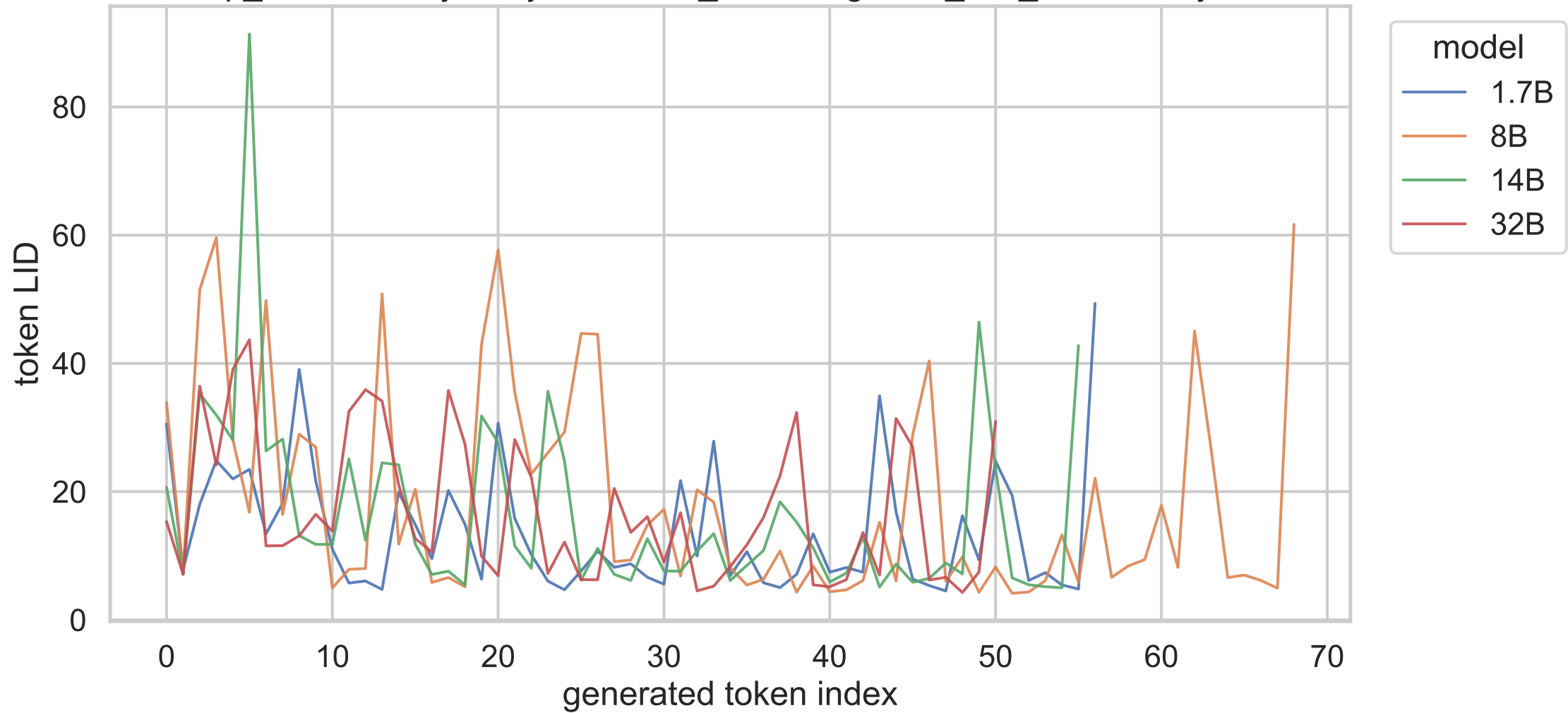
exp_b shared trajectory, irrelevant_context, gsm8k_test_000052, layer 6
