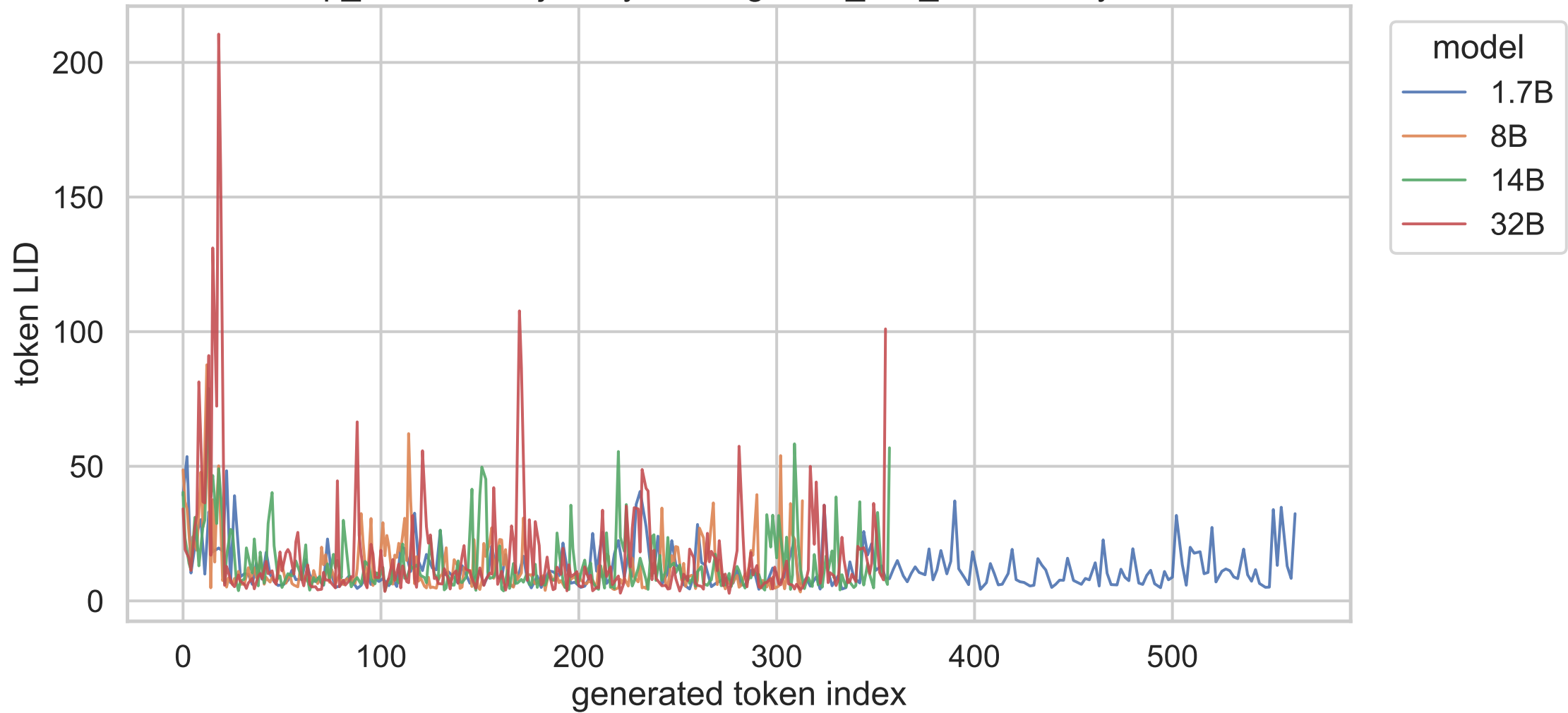
exp_c shared trajectory, think, gsm8k_test_000031, layer 13
