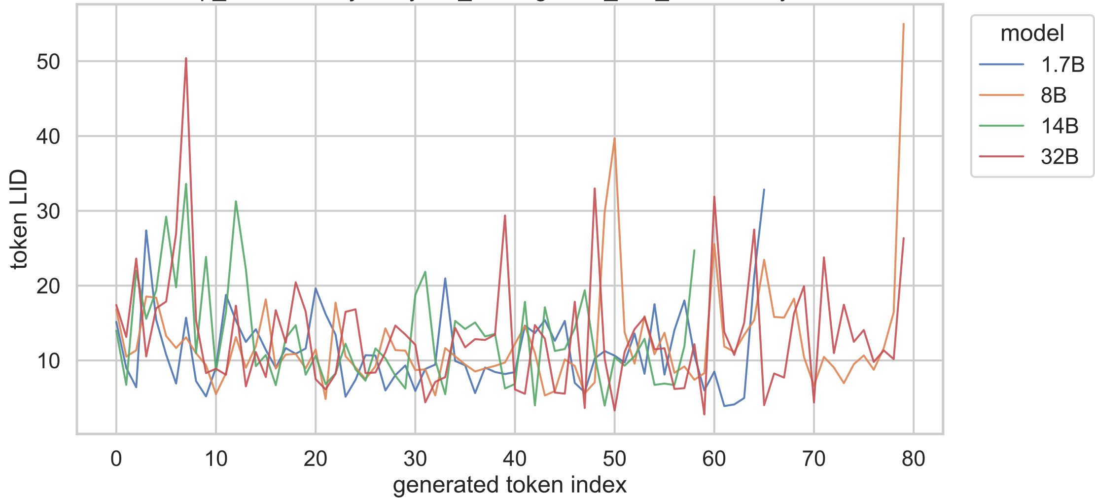
exp_c shared trajectory, no_think, gsm8k_test_000031, layer 20
