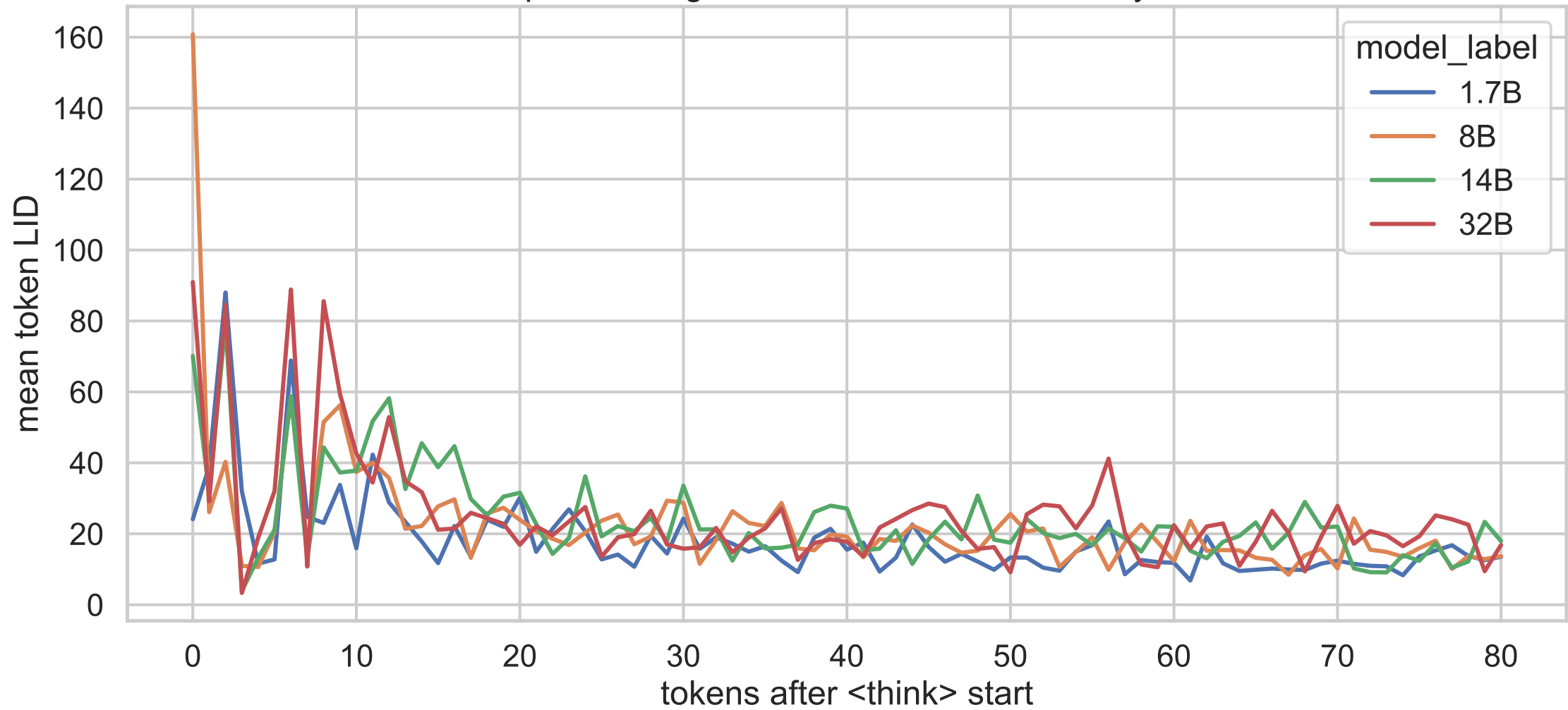
Exp C thinking-start anchored mean LID, layer 6
