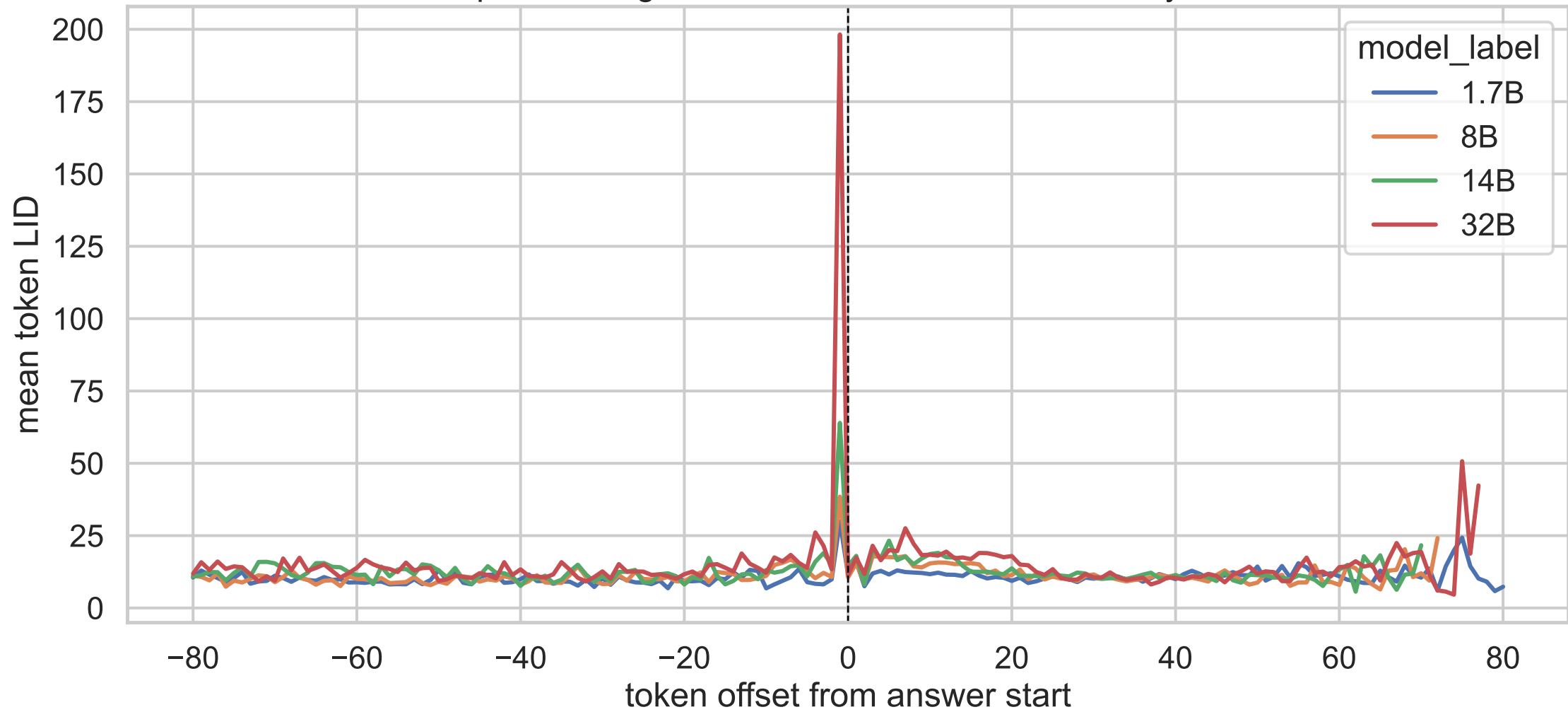
Exp C thinking-to-answer transition mean LID, layer 13
