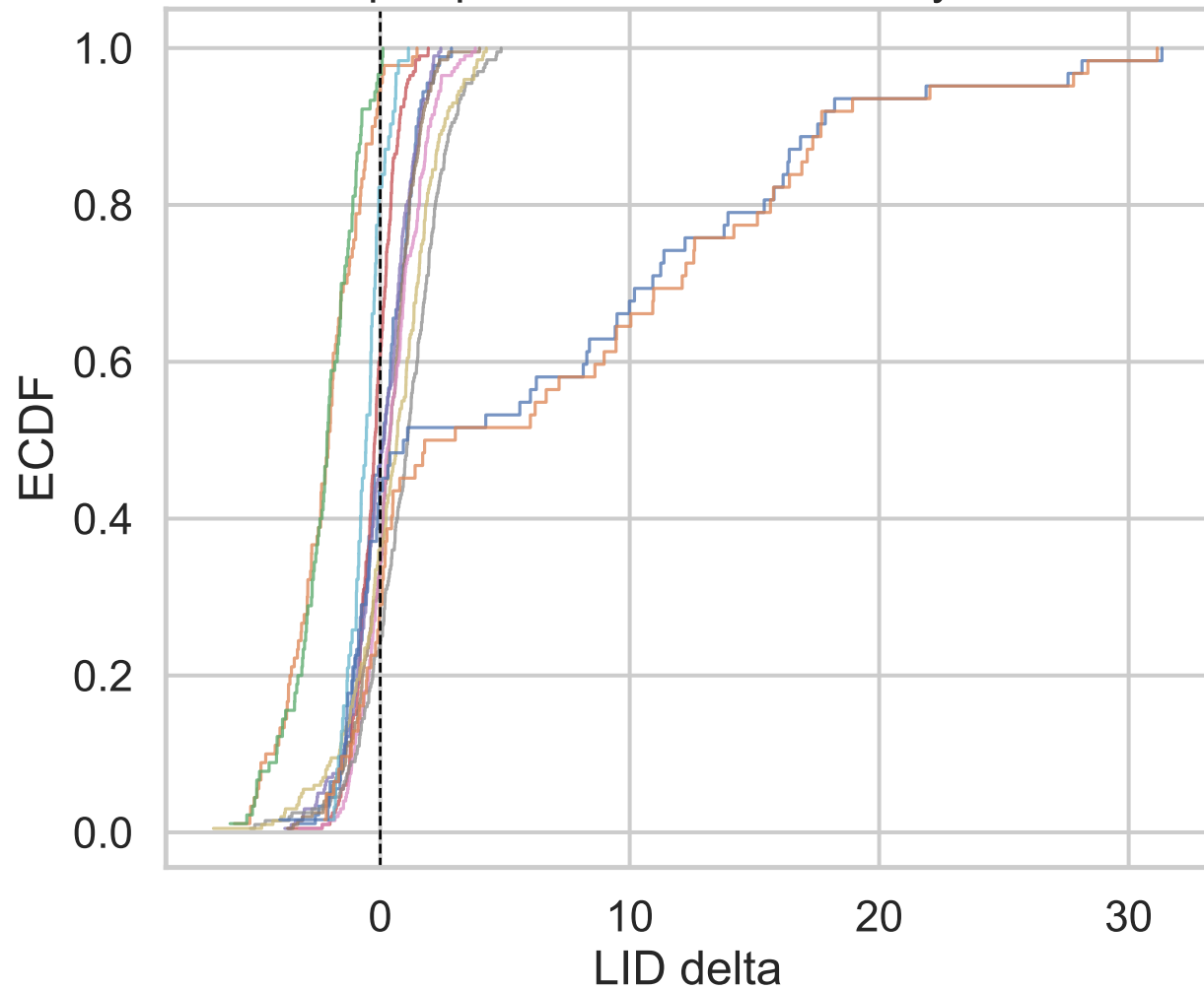
Exp C paired delta ECDFs, layer 20
