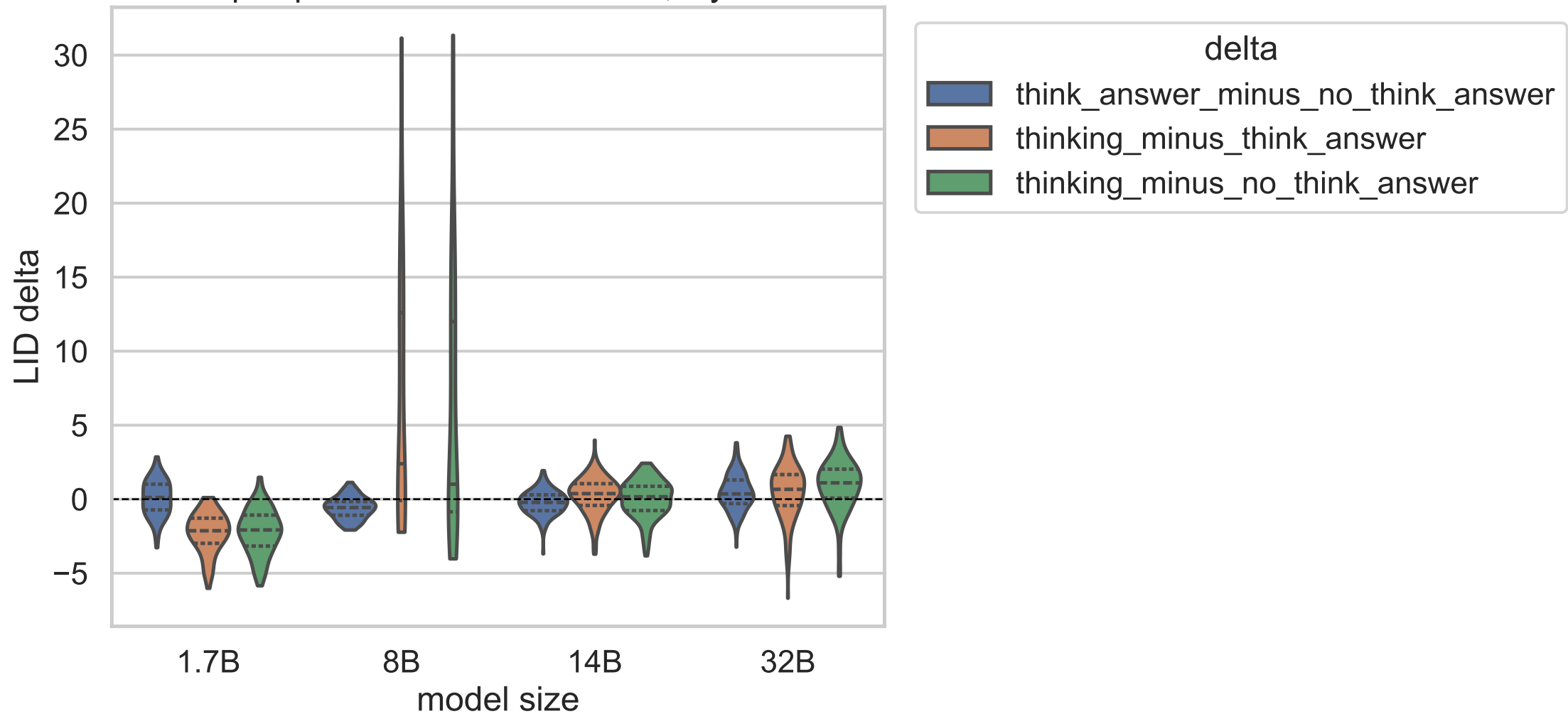
Exp C paired delta distributions, layer 20
