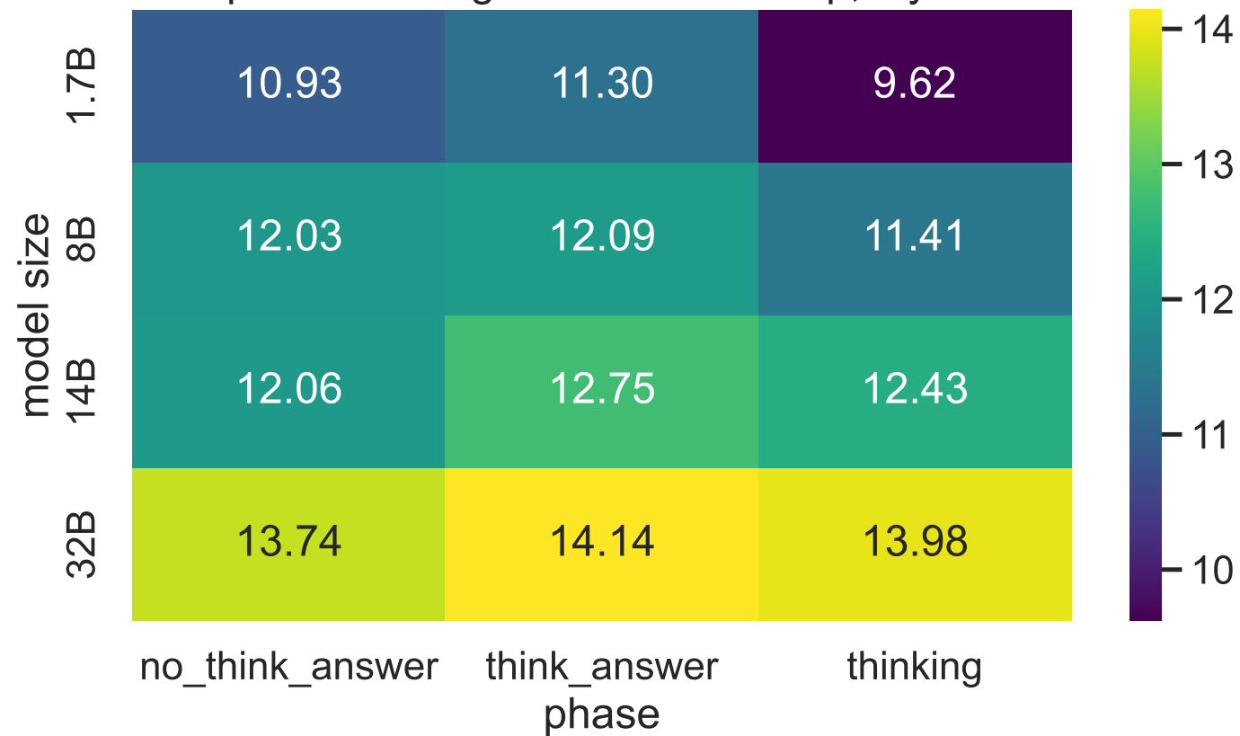
Exp C mean segment LID heatmap, layer 13
