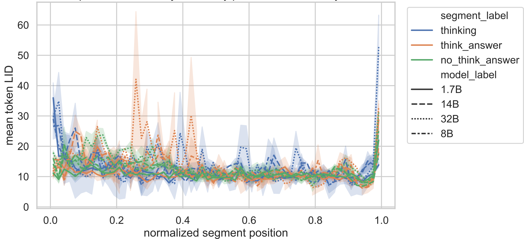
Exp C normalized trajectories by phase and model, layer 13
