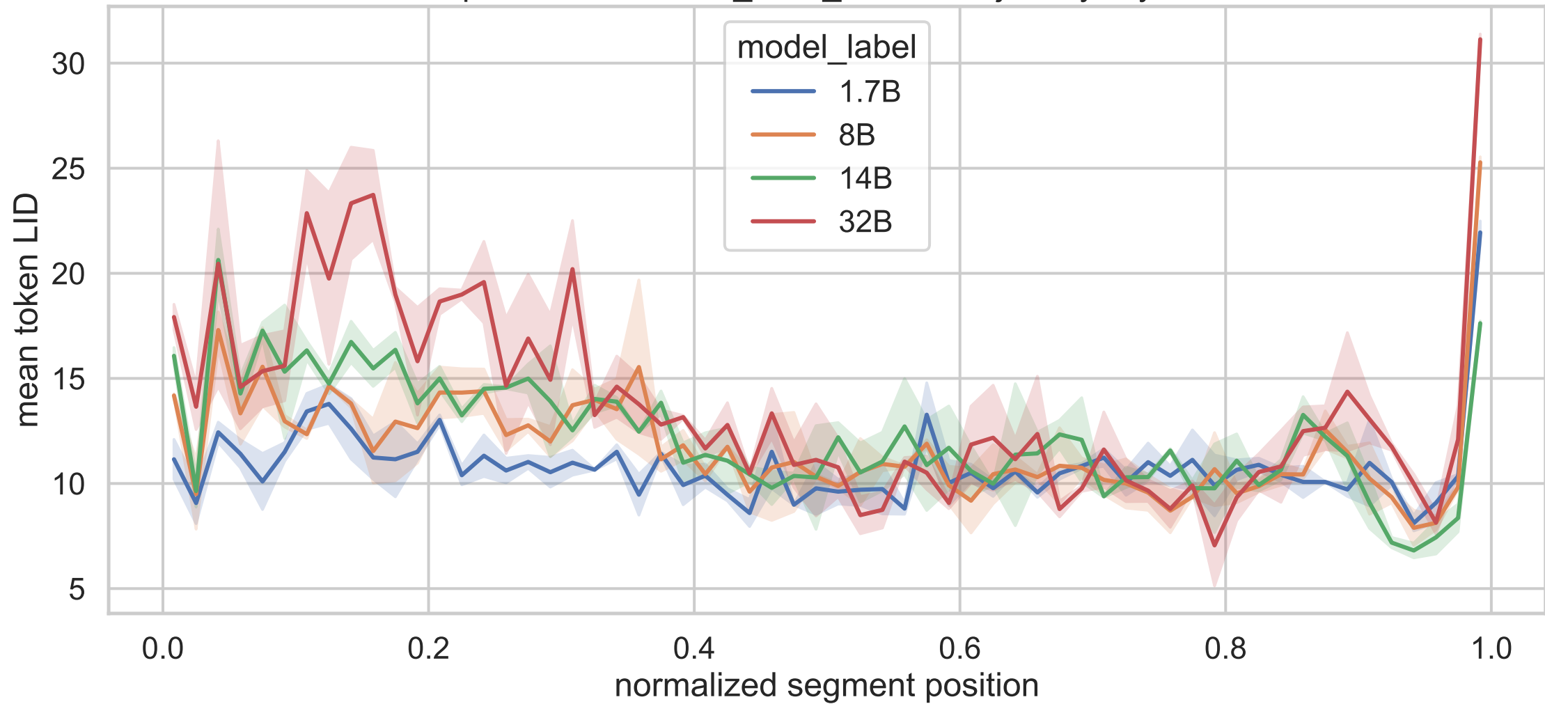
Exp C normalized no_think_answer trajectory, layer 13
