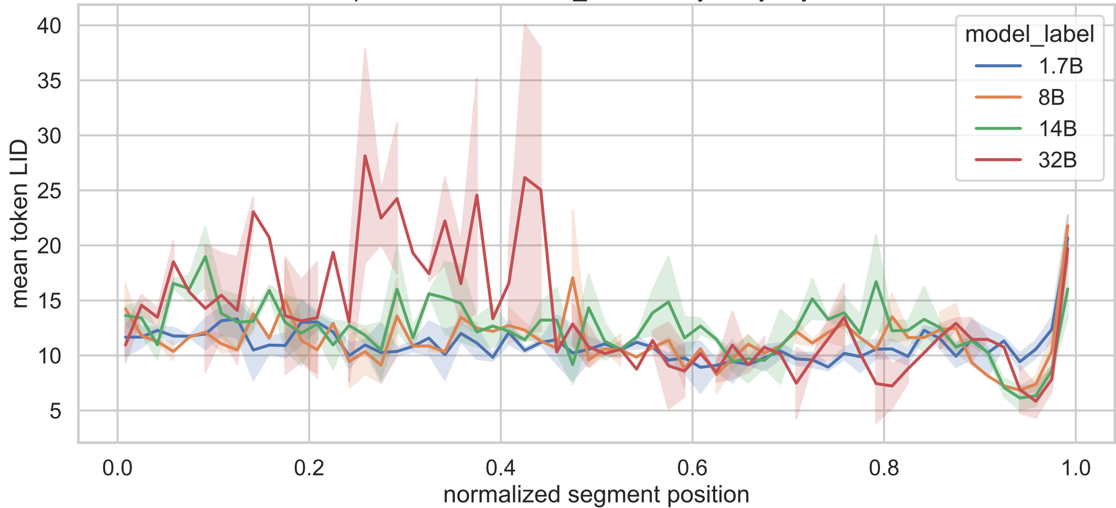
Exp C normalized think_answer trajectory, layer 20
