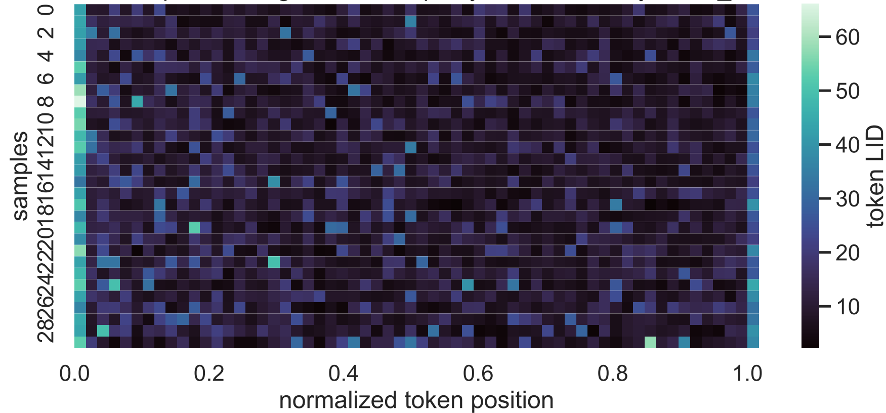
1.7B Exp C thinking LID heatmap, layer 13, sorted by mean_lid
