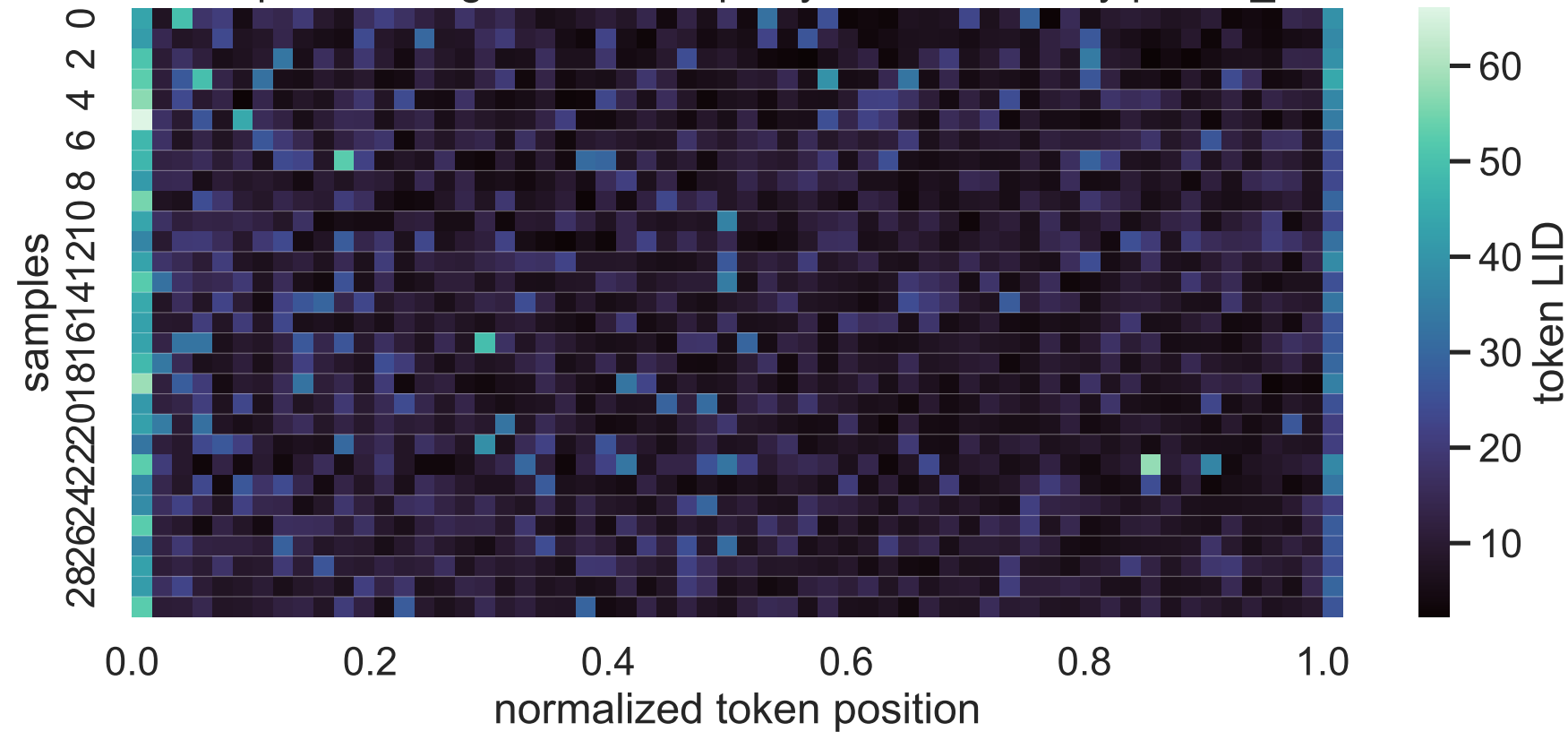
1.7B Exp C thinking LID heatmap, layer 13, sorted by paired_delta
