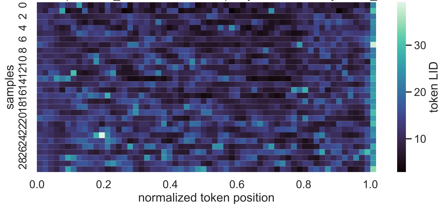
1.7B Exp C think_answer LID heatmap, layer 20, sorted by mean_lid
