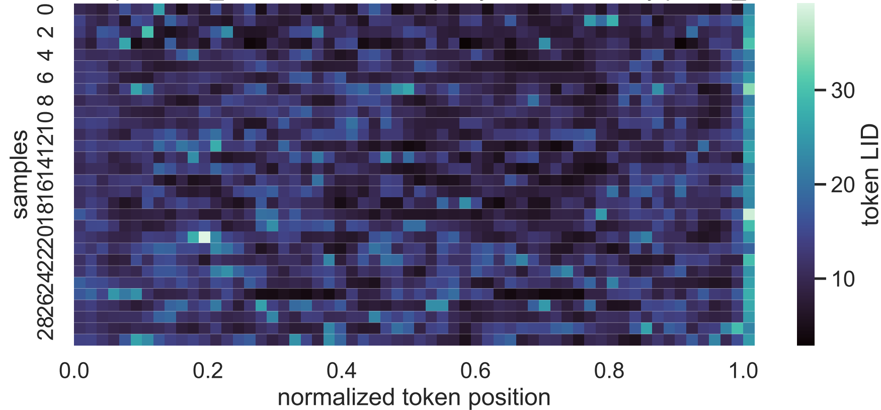
1.7B Exp C think_answer LID heatmap, layer 20, sorted by paired_delta
