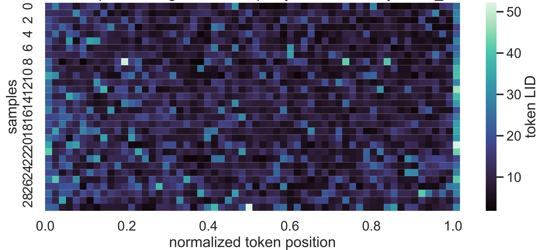
1.7B Exp C thinking LID heatmap, layer 20, sorted by mean_lid
