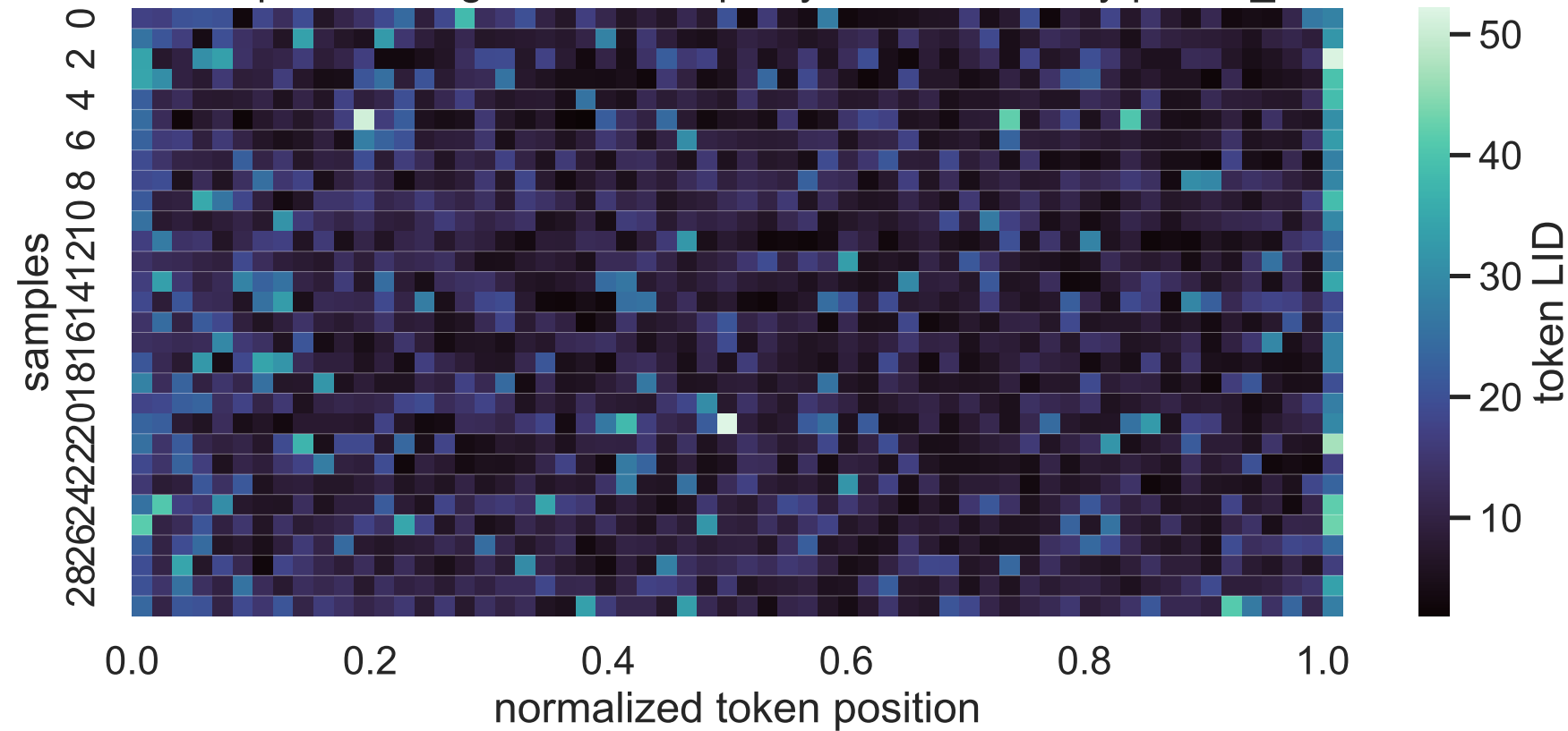
1.7B Exp C thinking LID heatmap, layer 20, sorted by paired_delta
